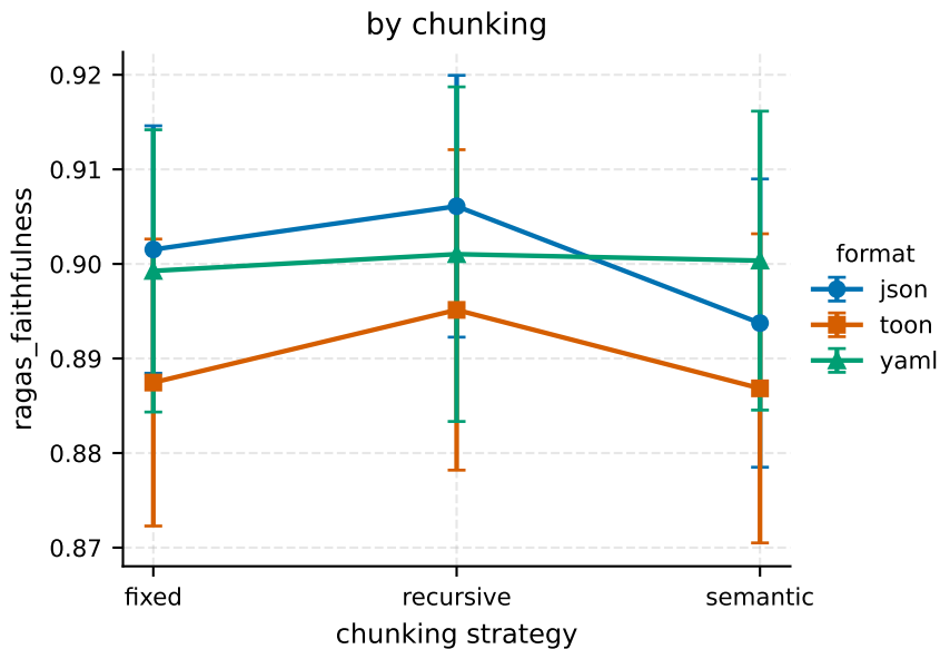
H2 — Format x chunking: no interaction (ragas_faithfulness ANOVA F=0.046, p=0.9960, ns)
