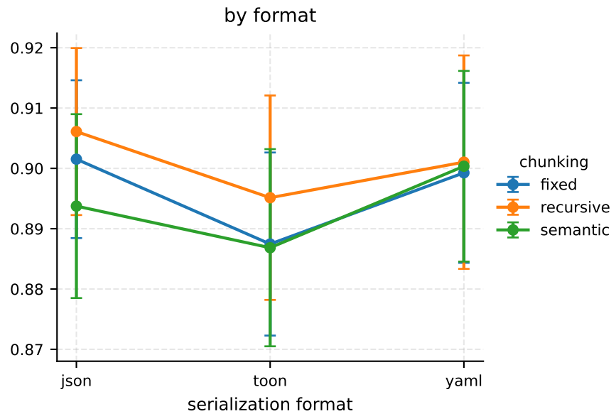
H2 — Format x chunking: no interaction (ragas_faithfulness ANOVA F=0.046, p=0.9960, ns)
