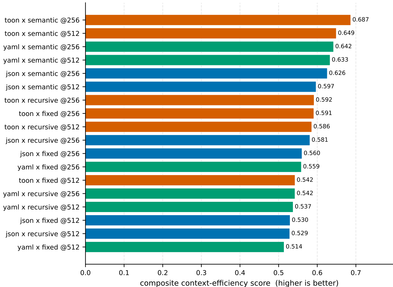
RQ5 — Configuration ranking
