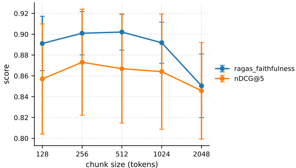
Fidelity vs chunk size
