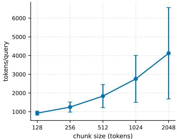
Prompt cost vs chunk size
