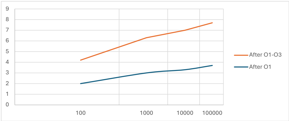
Figure 4: Scaling: Speedup of Optimizations on GPU
