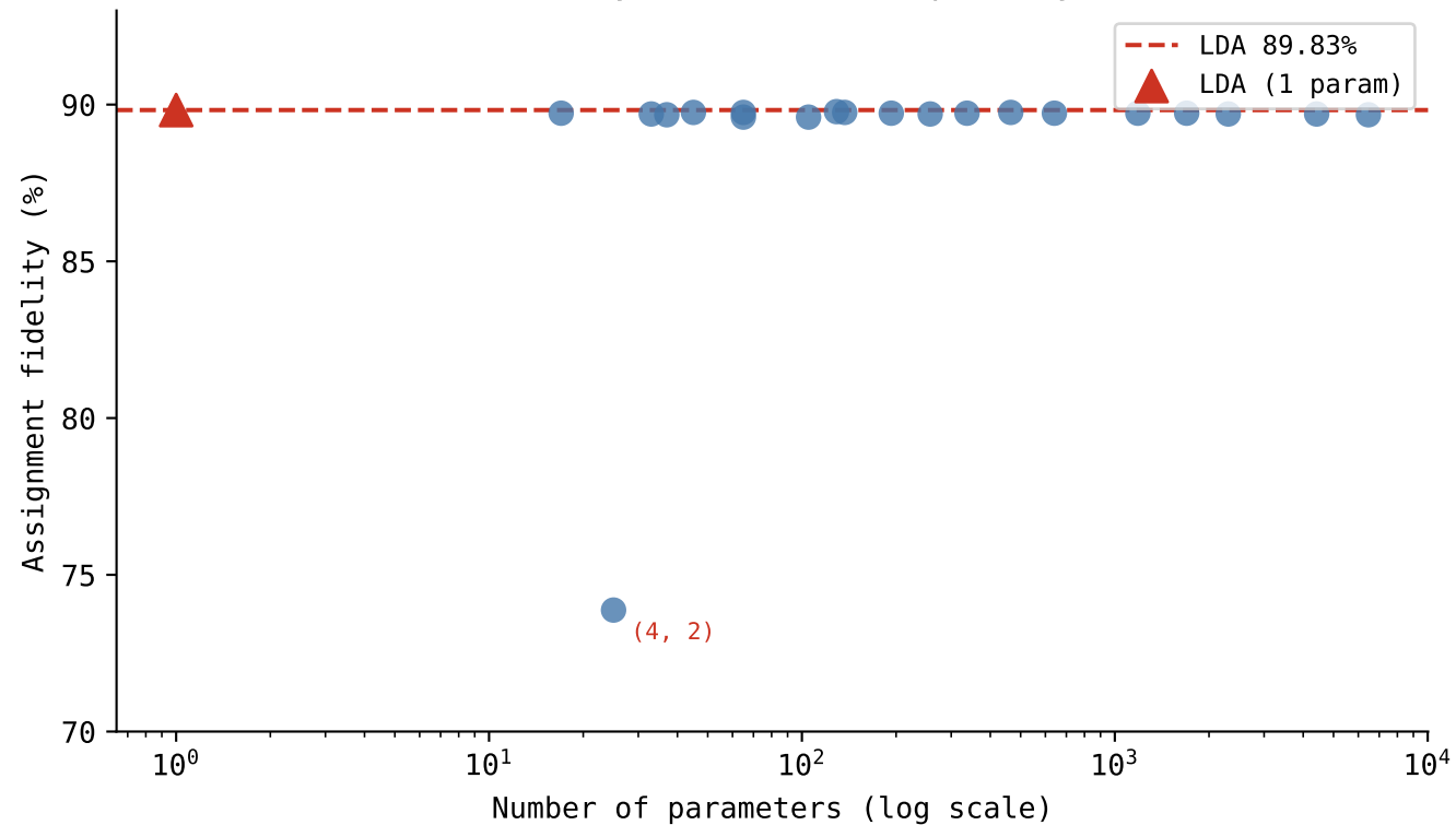
Fidelity vs. model complexity
