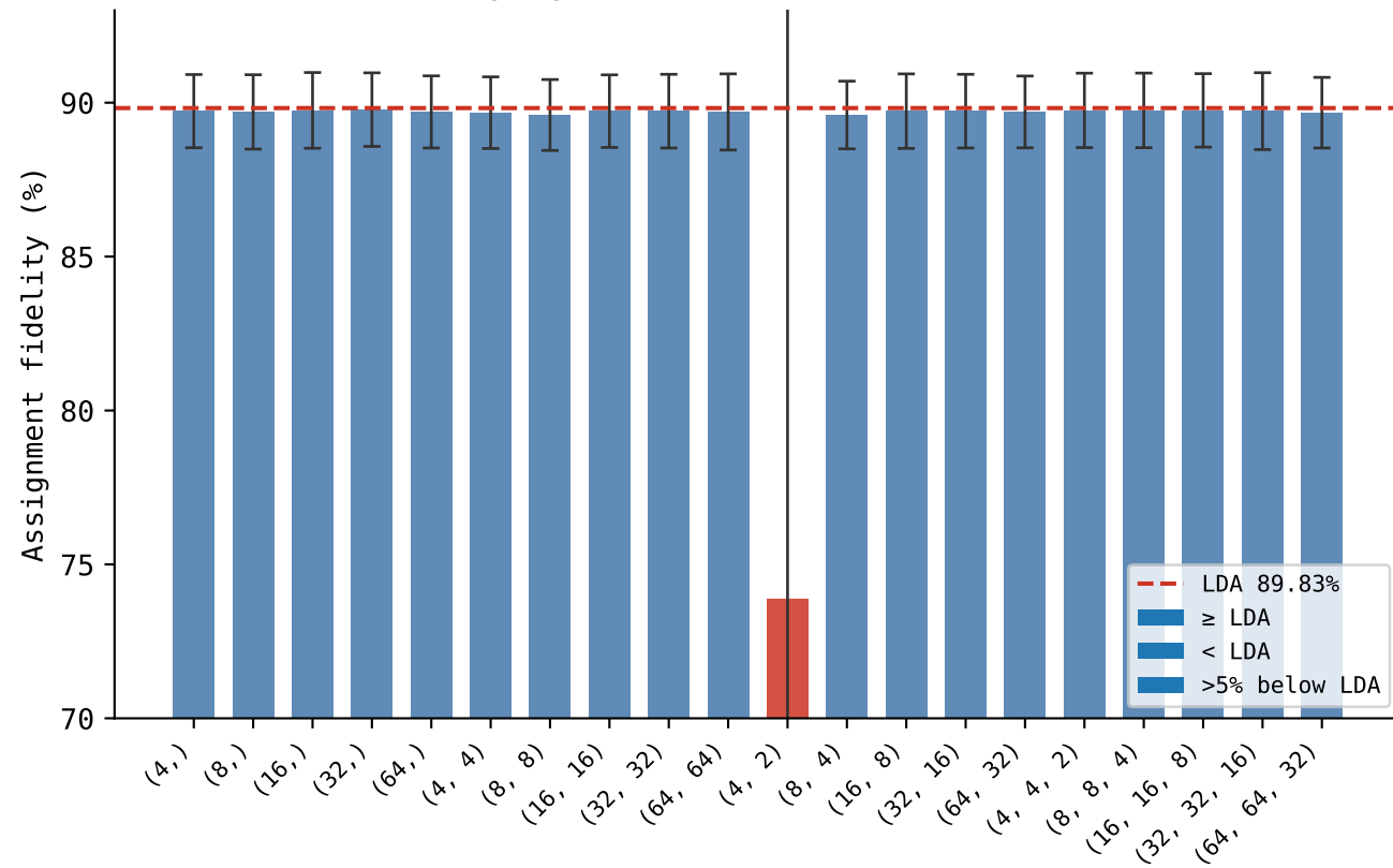
Fidelity by MLP architecture (5-fold CV)
