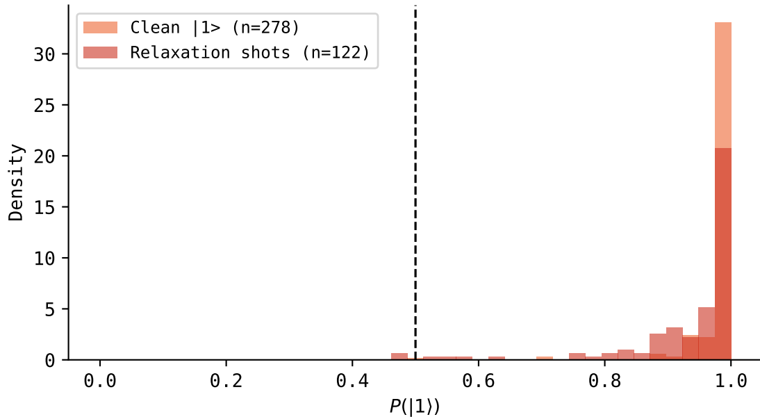
CNN confidence: clean vs. relaxation shots
