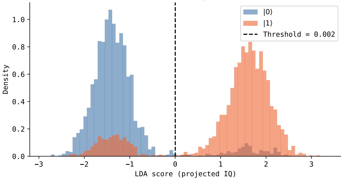
1D LDA Projection – histogram of shot scores
