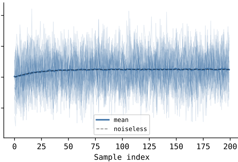
|1\rangle — Q channel
