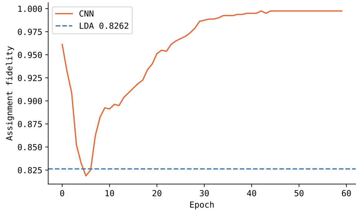
Test fidelity vs. LDA baseline
