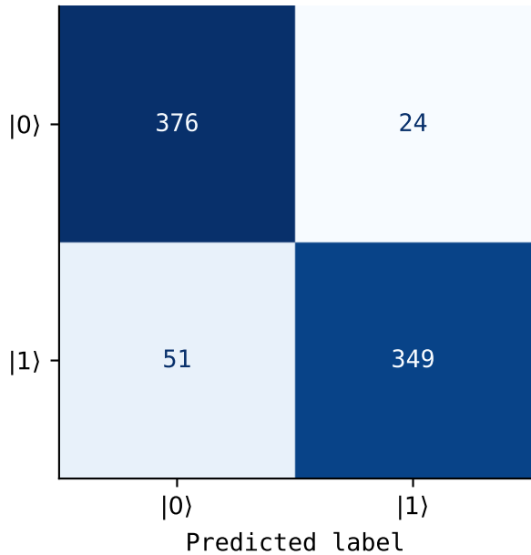
LDA
