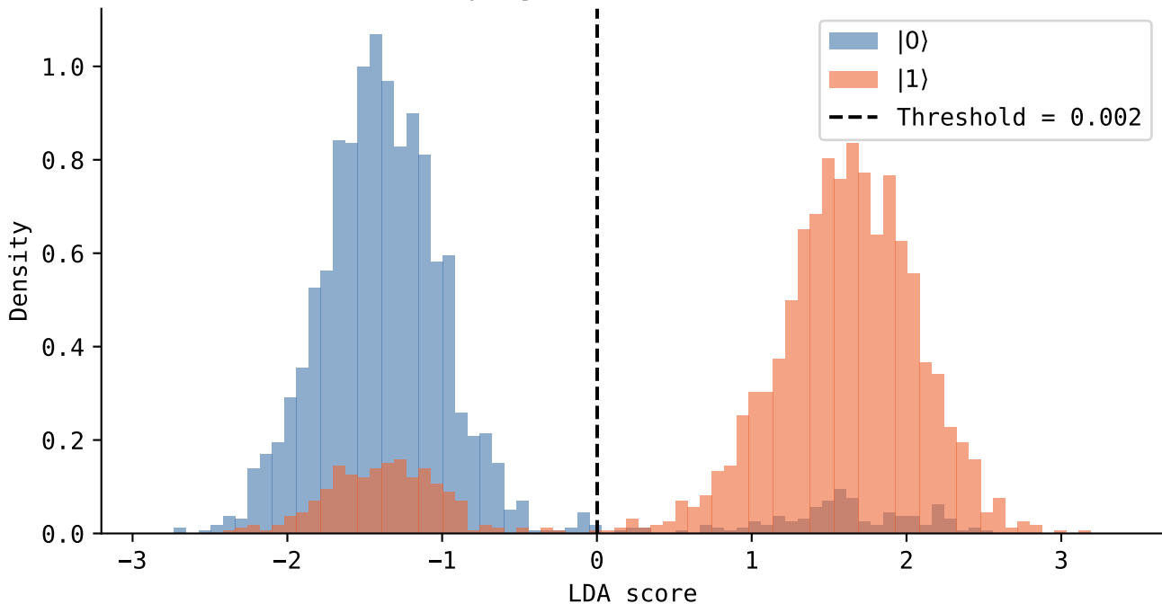
1D LDA projection — SNR = 2.464
