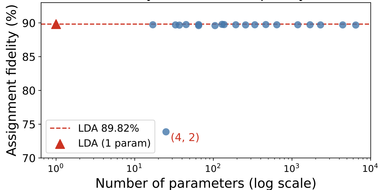
Fidelity vs. model complexity
