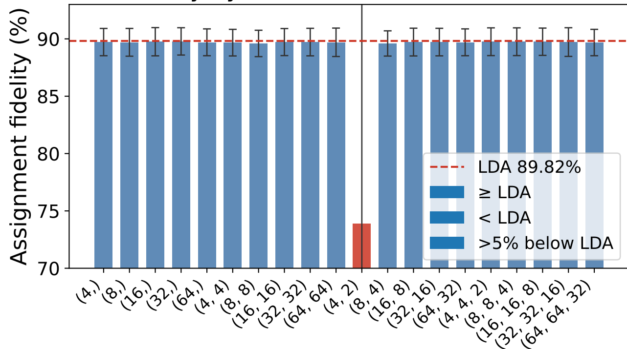
Fidelity by MLP architecture (5-fold CV)
