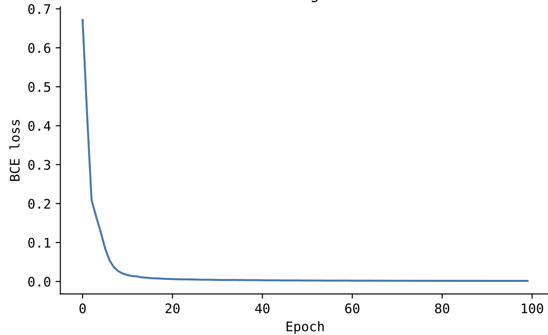
Training loss
