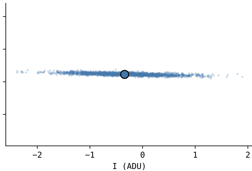
|1\rangle — IQ scatter (integrated)
