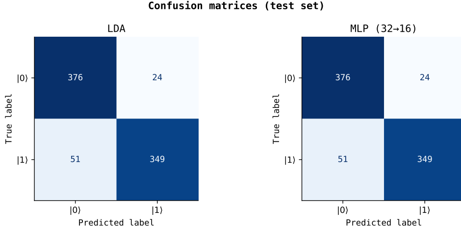
Figure 3: Confusion matrices for LDA and MLP (32 \rightarrow 16) on the held-out test set (800 shots). Both classifiers produce identical assignments: 376/400 correct for |0\rangle and 349/400 correct for |1\rangle . QDA produces the same matrix and is omitted. The asymmetry between off-diagonal entries (24 vs. 51) is the signature of T_1 relaxation biasing errors toward |1\rangle \rightarrow |0\rangle misclassification.
