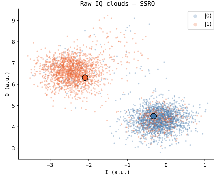
Figure 2: IQ scatter plot of the SSR0.h5 dataset (2000 shots per state). Blue: |0\rangle ; orange: |1\rangle . Filled circles mark the cluster centroids. The two clouds are well-separated and approximately Gaussian, with the |1\rangle ellipse visibly wider, consistent with the \approx 1.7\times covariance asymmetry in Table 4. The diagonal orientation of both ellipses reflects the residual IQ rotation noted in the text.
