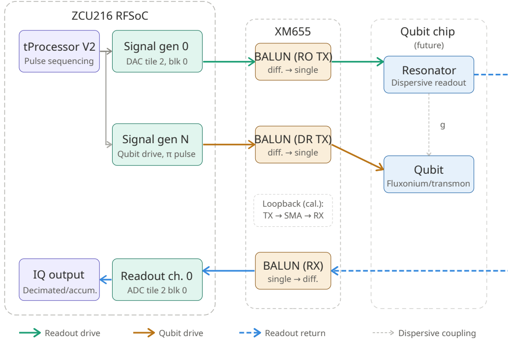
Figure 1: System signal chain for the QICK-based readout platform. The tProcessor V2 sequences pulses on two generator channels: the readout generator drives the readout tone through the XM655 TX BALUN to the resonator, and a second generator drives the qubit directly via a second TX BALUN channel for \pi -pulse control. The reflected readout tone returns through the XM655 RX BALUN to the readout ADC and is demodulated to an IQ pair (the channel and port numbers are those of Table 2). The XM655 BALUNs cover 10 MHz to 6000 MHz; resonator frequencies above 6 GHz require direct HD-header pigtail connections, bypassing the XM655. The qubit chip and its connections are shown as a design target; the board was not connected to a qubit chip within the scope of this work. Calibration experiments use the loopback path (TX BALUN \rightarrow SMA cable \rightarrow RX BALUN) shown inside the XM655 container.
