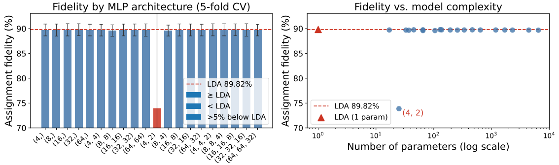
Figure 3: Architecture grid search results on integrated IQ data (5-fold CV). Left : assignment fidelity per MLP architecture; the red dashed line is the LDA baseline (89.82%). All architectures except the degenerate (4, 2) configuration lie within CV noise of LDA. Right : fidelity vs. parameter count on a log scale. No trend with model size is visible across three orders of magnitude. The one outlier, the (4, 2) architecture (a 4-neuron layer feeding a 2-neuron layer), sits at \approx 74\% with a large cross-validation spread ( \pm 0.20 ): the two-neuron bottleneck trains unstably, collapsing on some folds rather than failing for lack of capacity. It is excluded from Table 6.
