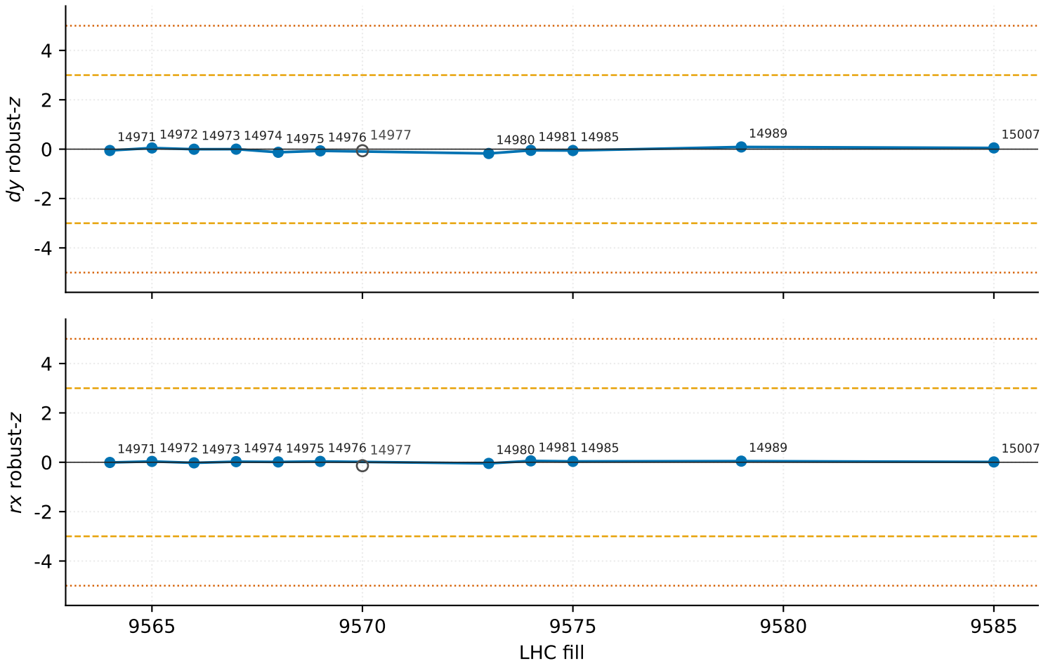
Isolation residuals vs frozen 14973/14974 scale (DQ observable)
