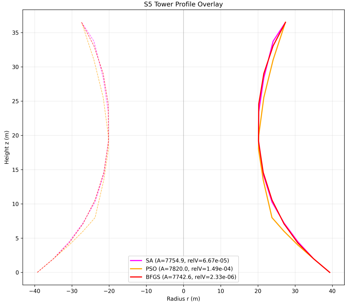
Figure 8.14: S5 profile
