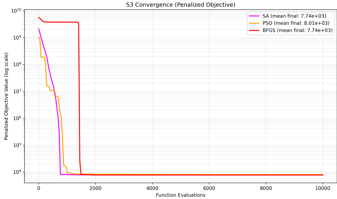
Figure 8.7: S3 convergence
