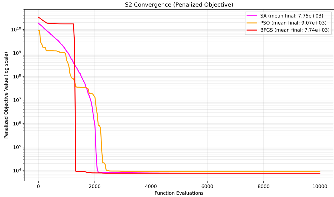
Figure 8.4: S2 convergence
