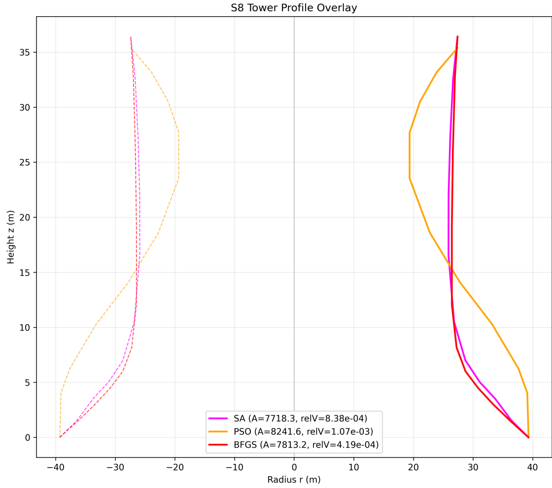
Figure 8.23: S8 profile
