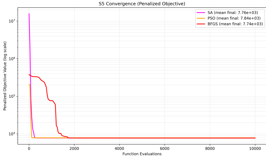
Figure 8.13: S5 convergence
