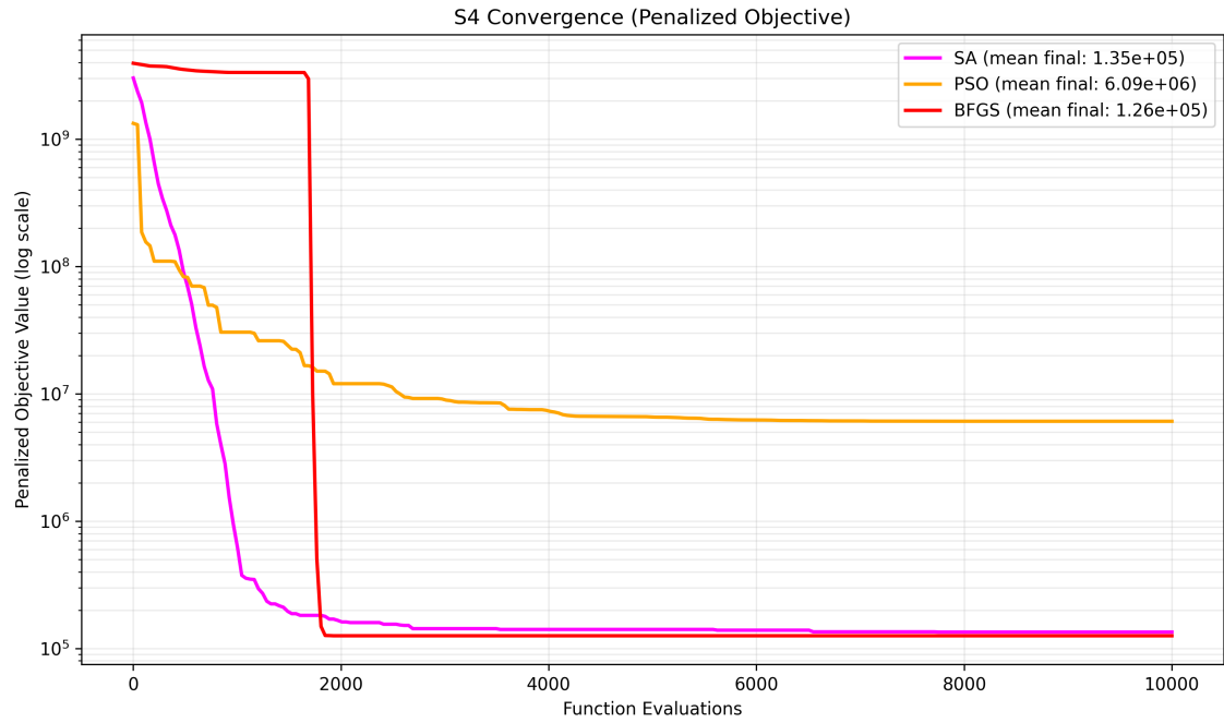
Figure 8.10: S4 convergence
