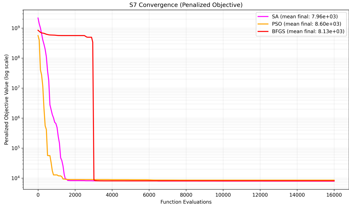
Figure 8.19: S7 convergence
