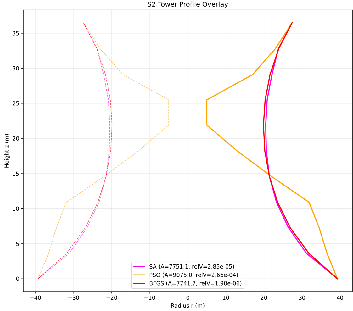
Figure 8.5: S2 profile
