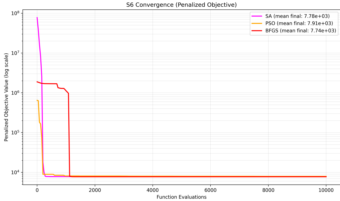
Figure 8.16: S6 convergence
