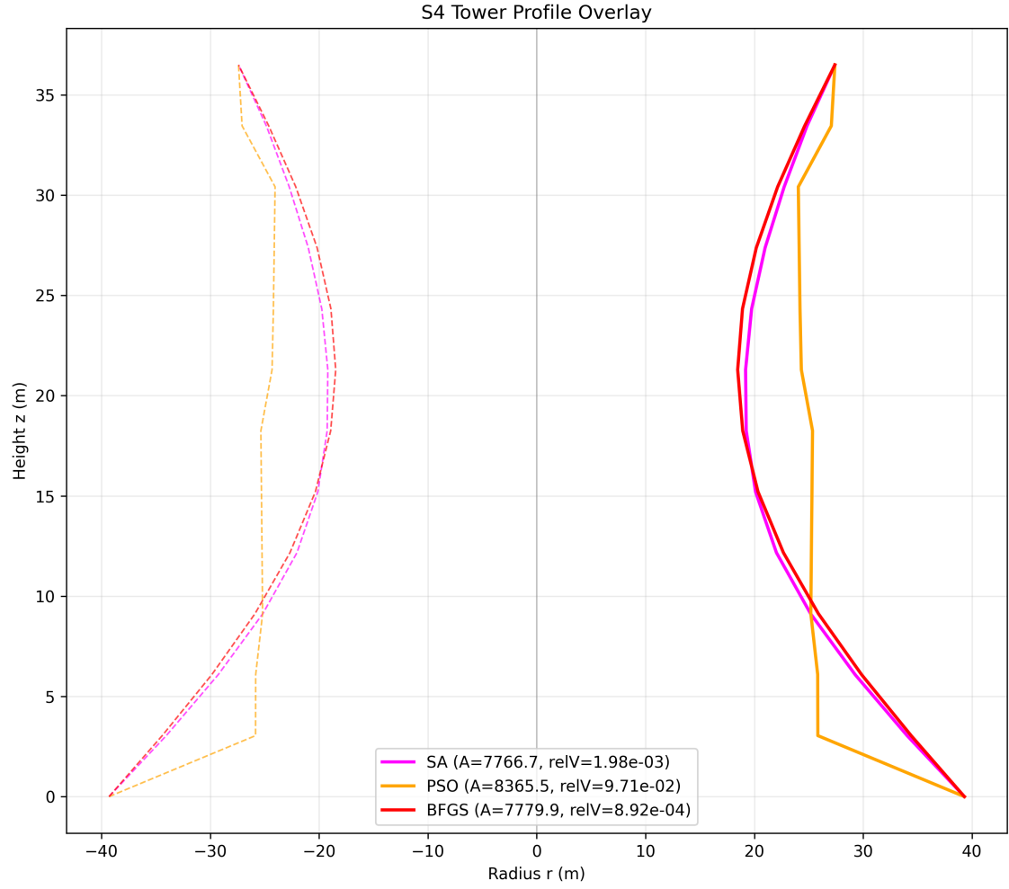
Figure 8.11: S4 profile
