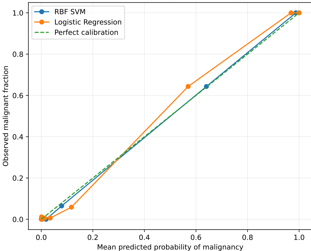
Calibration of the two highest-ranked algorithms
