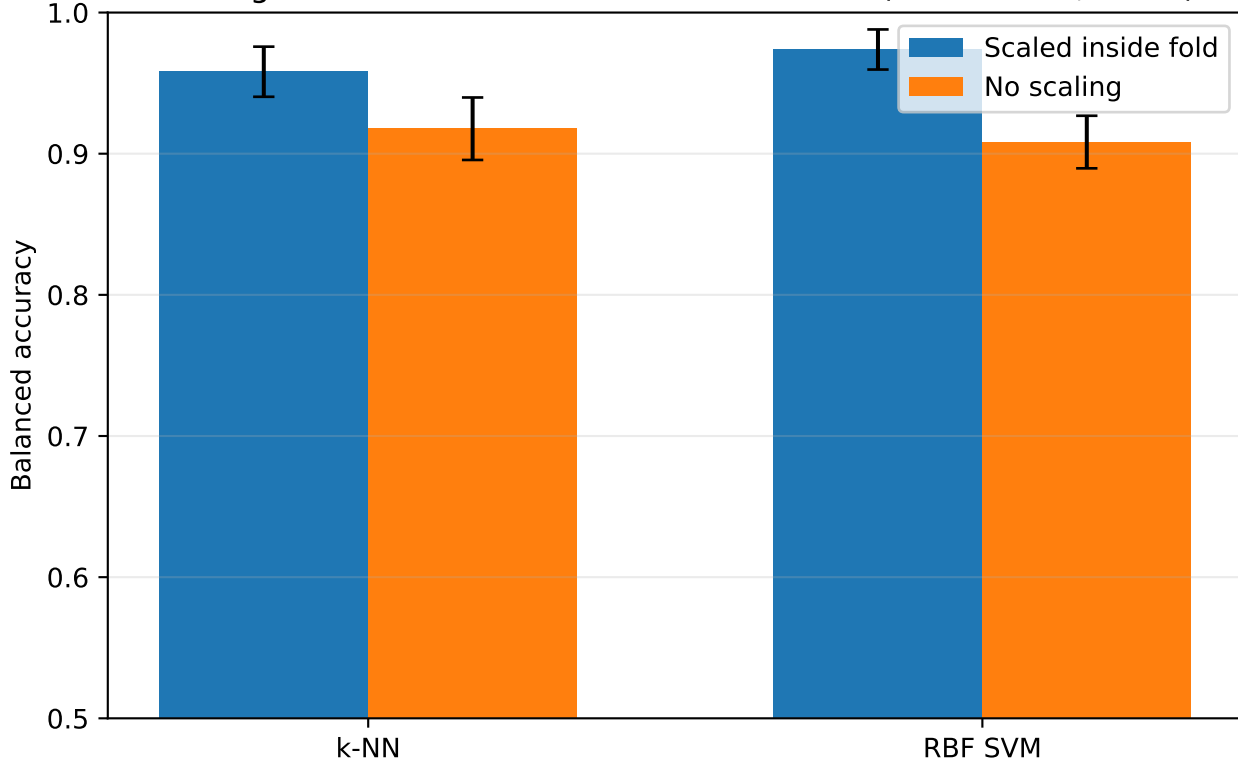
Scaling ablation for distance/kernel methods (mean \pm SD, n=15)
