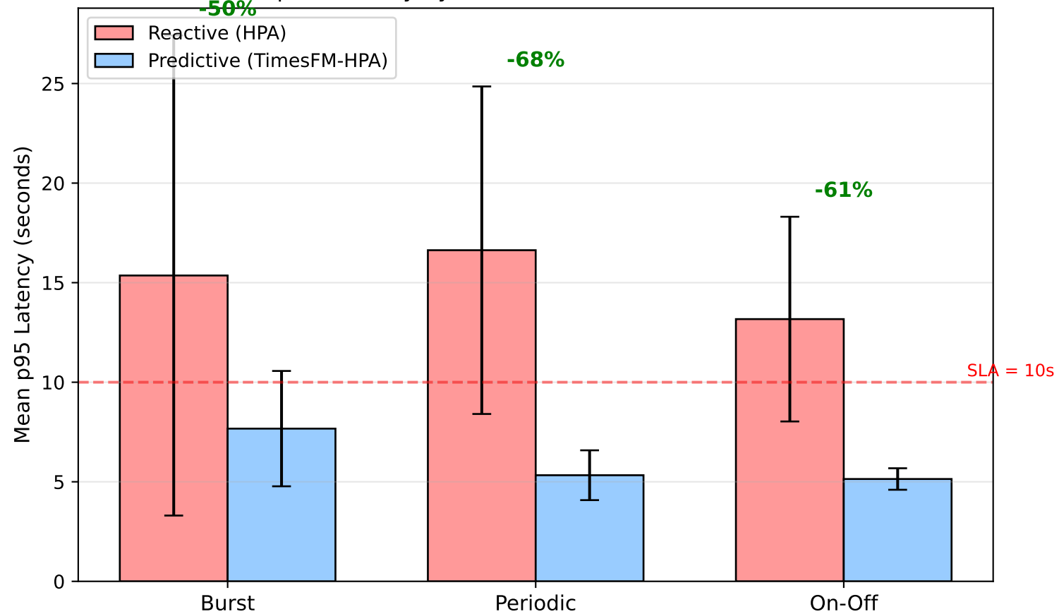
Mean p95 Latency by Workload (error bars: \pm 1 SD, n=10)
