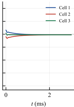
With balancing (controller I)
