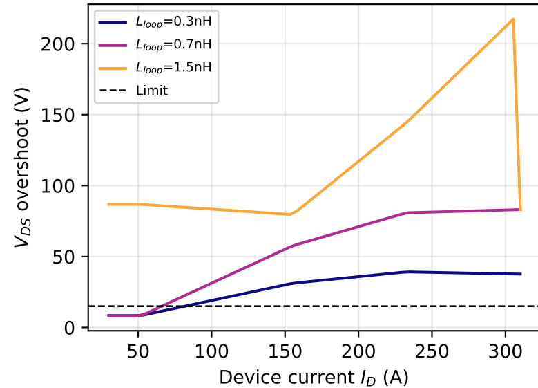
Overshoot, R_g=2\Omega
