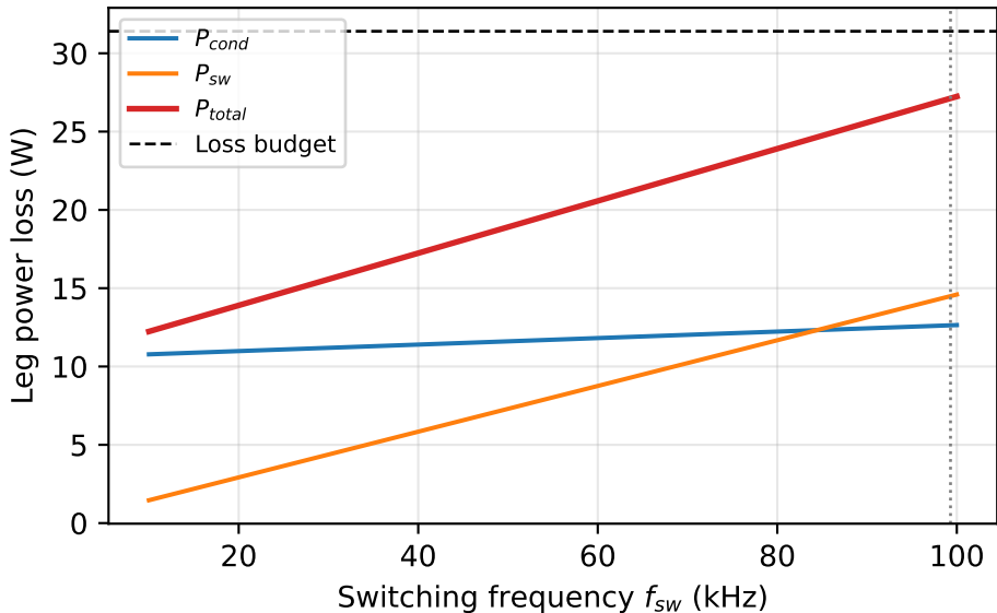
Loss vs. f_{sw} at N=4 , R_g=(0.5/2.7)\Omega
