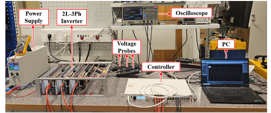
Fig. 8. Experimental setup of 2-Level 3-Phase Inverter System.
