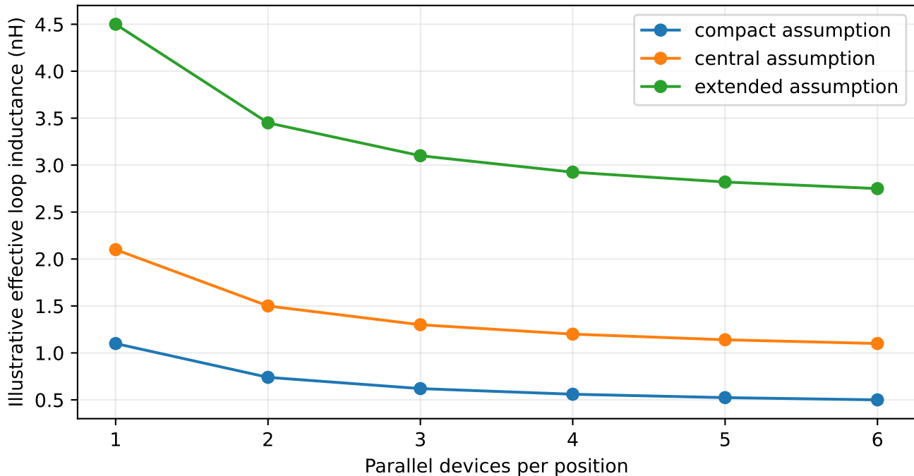
Assumed symmetric branches: shared inductance limits improvement
