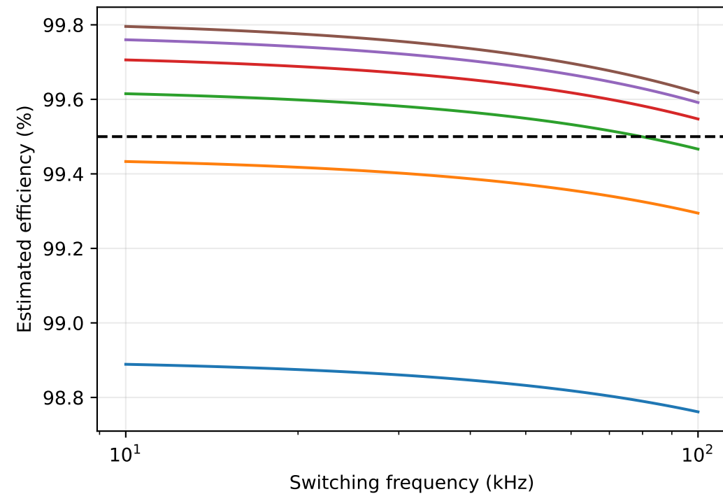
75 V SPB inverter module - preliminary screening, assumed timing
