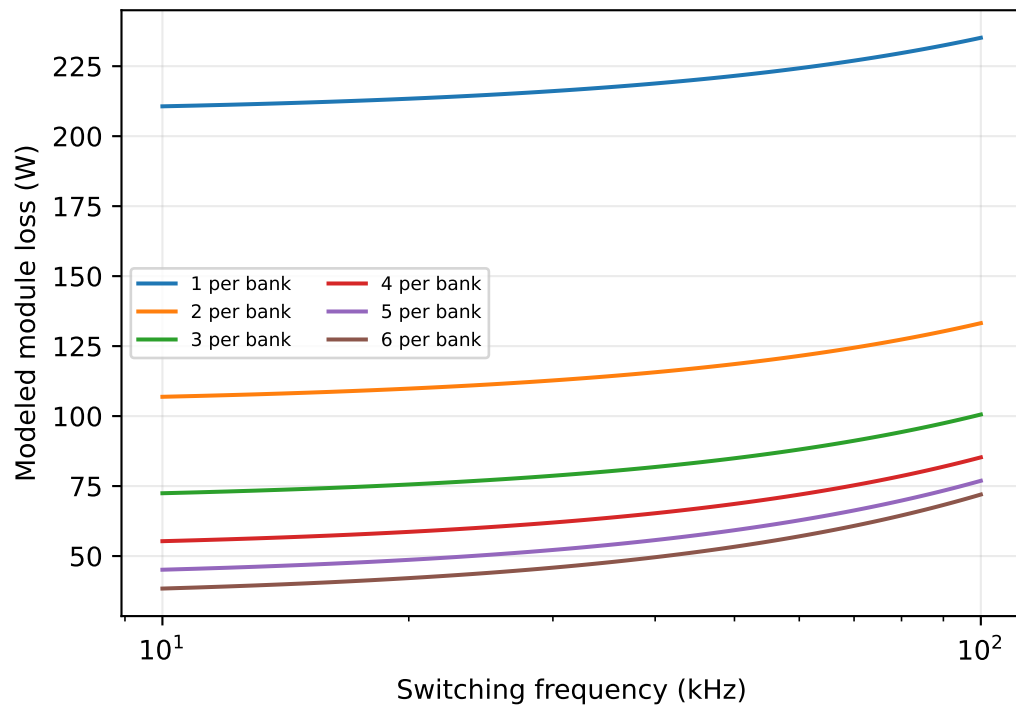
75 V SPB inverter module - preliminary screening, assumed timing
