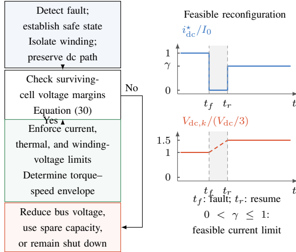
FIGURE 15. Post-fault feasibility assessment with illustrative waveforms for the feasible branch. The dc-current command is temporarily set to zero and restored to \gamma I_0 , subject to operating limits. For a fixed bus, changing from three to two active cells raises the balanced surviving-cell voltage from 1 to 1.5 p.u. (400 to 600 V for a 1200-V bus). Shading marks the protection/reconfiguration interval; the dashed voltage connection indicates a change of steady-state level, not a predicted capacitor-voltage trajectory. Current derating does not remove the increased blocking-voltage requirement.
