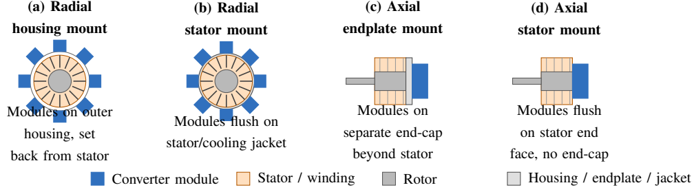
FIGURE 7. Physical integration options for SPB-compatible converter modules on a radial-flux machine, following the four-category taxonomy of [79]: (a) radial housing mount, (b) radial stator mount, (c) axial endplate mount, and (d) axial stator mount, each shown in whichever radial or axial cross-section most clearly conveys its mounting geometry.
