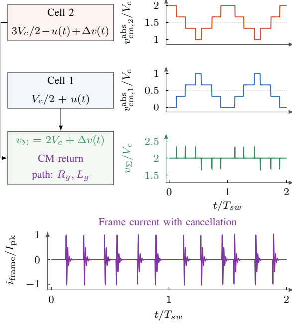
FIGURE 11. Nonideal two-cell common-mode cancellation over two switching periods. Small transition misalignment produces narrow residuals in v_\Sigma ( t_d/T_{sw} = 0.003 , t_r/T_{sw} = 0.004 ). Their polarities follow the three rising and three falling cell-voltage transitions; unequal dv/dt can also produce residuals. The lower plot shows damped frame current with cancellation, normalized to its own peak I_{pk} . For equal winding-to-frame capacitances C_g and a shared frame-to-ground return impedance R_g + sL_g , I_{frame}(s)/V_\Sigma(s) = sC_g/(1 + 2R_gC_g s + 2L_gC_g s^2) . The illustrative resonance has f_0/f_{sw} = 65 and damping ratio \zeta = 0.22 . Each residual excites alternating-polarity current ringing. This lumped-model illustration excludes shaft charging and bearing-film breakdown; it is not a bearing-discharge prediction.
