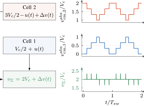
FIGURE 11. Nonideal two-cell common-mode cancellation over two switching periods. Small transition misalignment produces narrow residuals in v_{\Sigma} .
