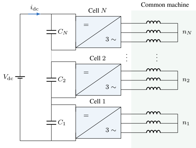
FIGURE 3. Conceptual architecture of an N -cell SPB traction drive: series-connected local dc-link capacitors, series-connected three-phase two-level bridge cells, and their electrically separated machine winding groups.
