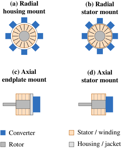
FIGURE 7. Physical integration options for a radial-flux machine, following [79].
