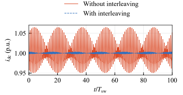
FIGURE 9. Analytical steady-state shared dc-link current for three identical SPB cells with ideal natural SPWM over one fundamental period. Parameters are M = 0.85 , power-factor angle 20^\circ , f_{sw}/f_1 = 100 , L_b C/T_{sw}^2 = 0.85 , and R_b C/T_{sw} = 2.5 .
