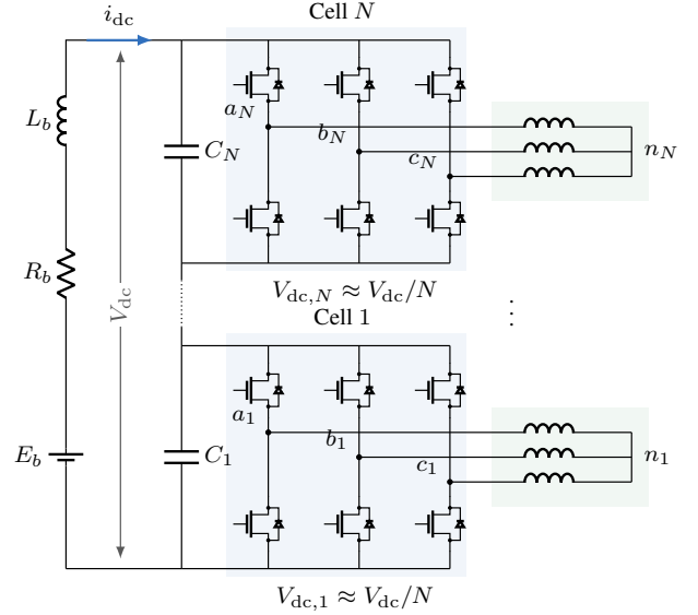
FIGURE 5. Switch-level realization of the SPB dc–ac stage for two representative cells (Cell 1 and Cell N ; cells 2, \dots, N-1 elided).
