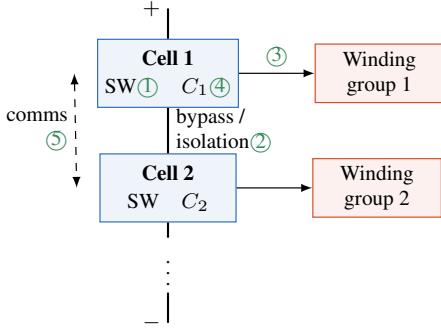
FIGURE 14. Simplified SPB converter-machine structure with fault locations ①–⑤ annotated, corresponding in order to the rows of Table 5.
