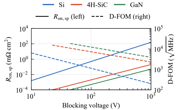
FIGURE 2. Ideal one-dimensional unipolar specific on-state resistance R_{on,sp} (solid, left axis) and the resulting high-frequency device figure-of-merit D-FOM = 1/\sqrt{R_{on,sp} C_{oss,sp}} (dashed, right axis), in \sqrt{MHz} – the product R_{on,sp} C_{oss,sp} is an area-independent RC time constant, versus blocking voltage for Si, 4H-SiC, and GaN.
