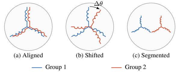
FIGURE 6. Schematic comparison of winding-group spatial arrangements: (a) aligned groups (parallel phase axes), (b) spatially shifted groups (offset by \Delta\theta ), and (c) physically segmented stator modules.
