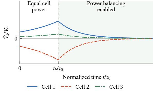
FIGURE 12. Conceptual analytical illustration of voltage balancing for three cells during motoring, based on (20) and [45]. Small deviations from the mean grow under equal constant cell powers. Enabling differential power balancing at t_b makes them decay toward zero while \sum_k \Delta P_k = 0 . Time is normalized by \tau_0 = CV_0/I_{dc,0} .
