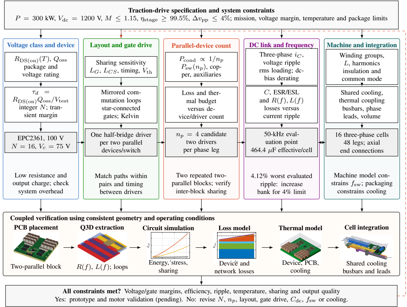
FIGURE 16. Iterative SPB system-design procedure with coupled verification and cell integration. Machine requirements feed back into switching-frequency, insulation, and thermal design. Original two-parallel building-block models support the four-parallel analytical projection; shared cooling and interconnections require assembly-level and experimental validation.
