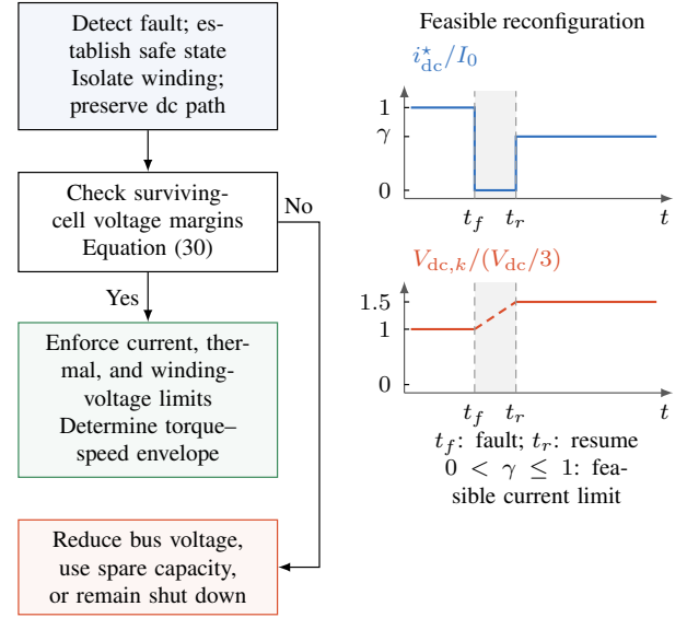
FIGURE 15. Post-fault feasibility assessment with illustrative waveforms for the feasible branch. The dc-current command is temporarily set to zero and restored to \gamma I_0 , subject to operating limits. For a fixed bus, changing from three to two active cells raises the balanced surviving-cell voltage from 1 to 1.5 p.u. (400 to 600 V for a 1200-V bus).
