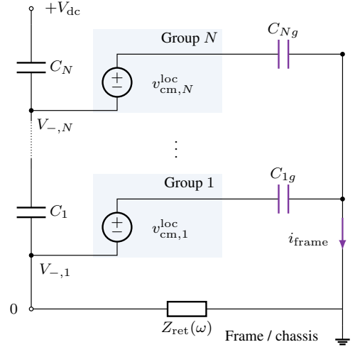
FIGURE 10. Lumped common-mode equivalent of the SPB stack.
