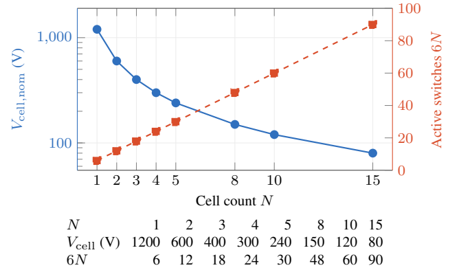
FIGURE 13. Cell-count scaling for a 1200-V dc link: nominal cell voltage V_{cell,nom} = V_{dc}/N and active switch positions 6N .
