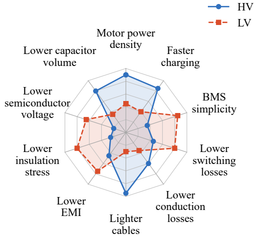
FIGURE 1. Conceptual illustration of qualitative system-level tradeoffs between low-voltage and high-voltage traction architectures.
