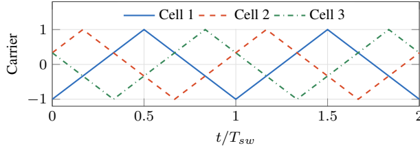
FIGURE 8. Uniform carrier interleaving for N = 3 , with phase offsets 0 , 2\pi/3 , and 4\pi/3 . Analytically generated triangular carriers.
