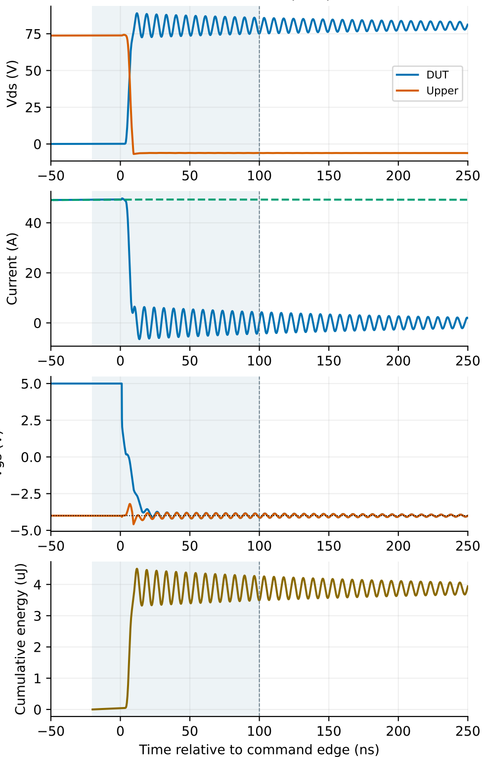
First turn-off (Eoff)
