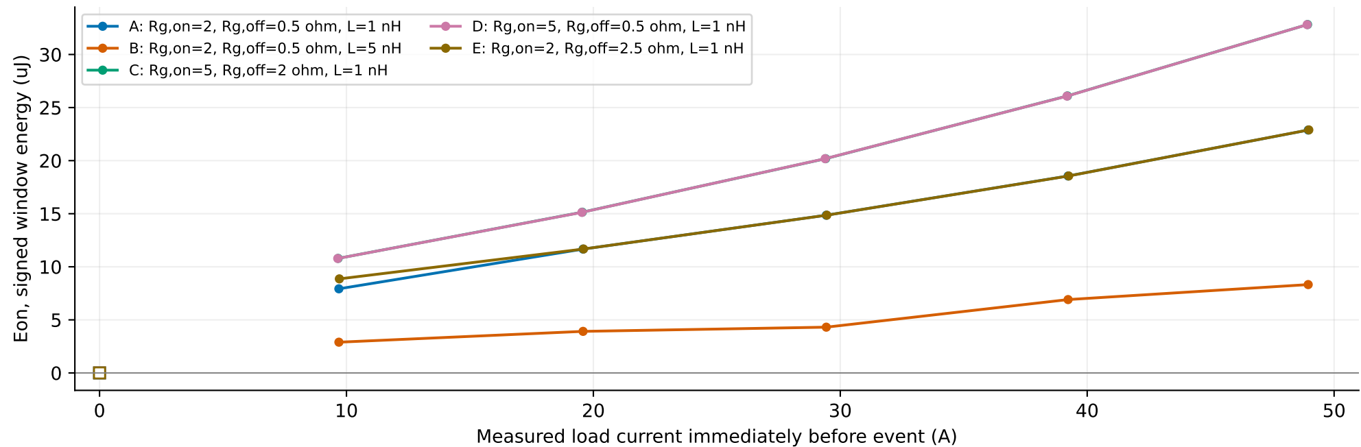
Switching-window energy vs current | -20 ns to +100 ns
