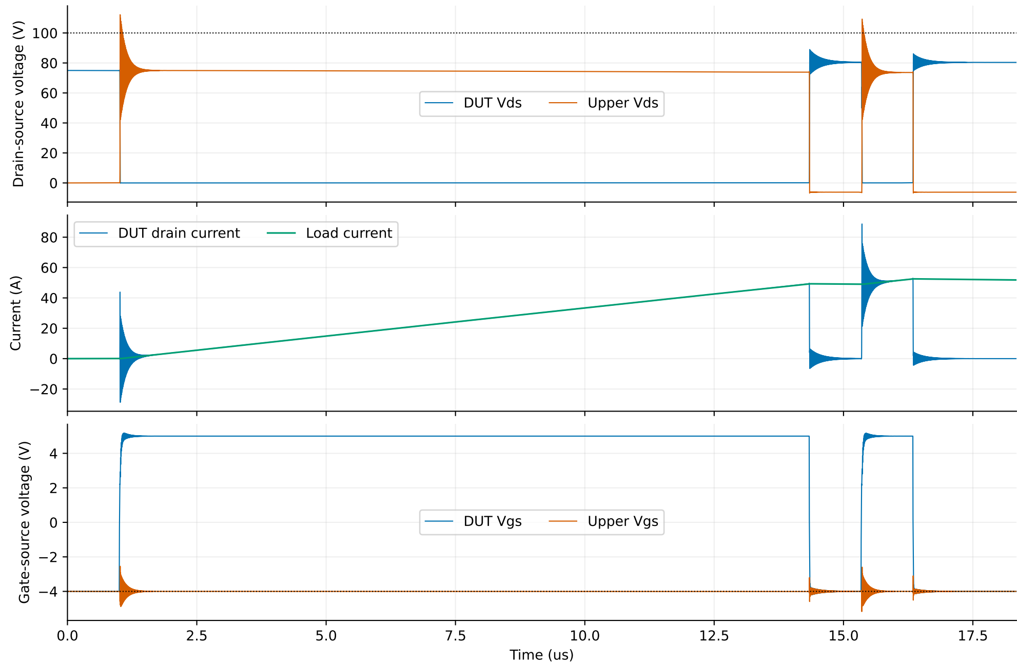
Configuration A | nominal 50 A | 75 V DC link | +5 / -4 V drive
