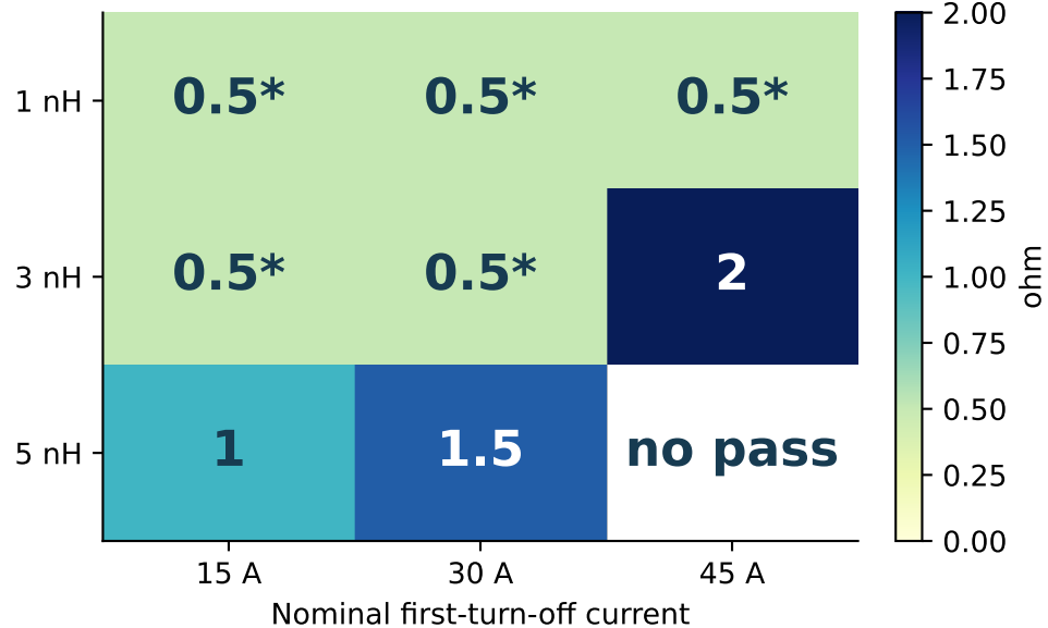
Selected external turn-off resistance
