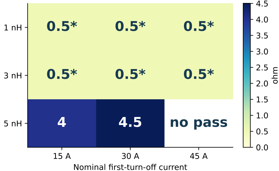
Selected external turn-on resistance
