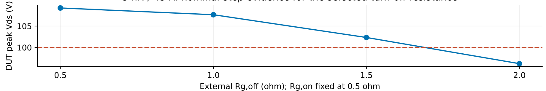
3 nH / 45 A: nominal-step evidence for the selected turn-off resistance
