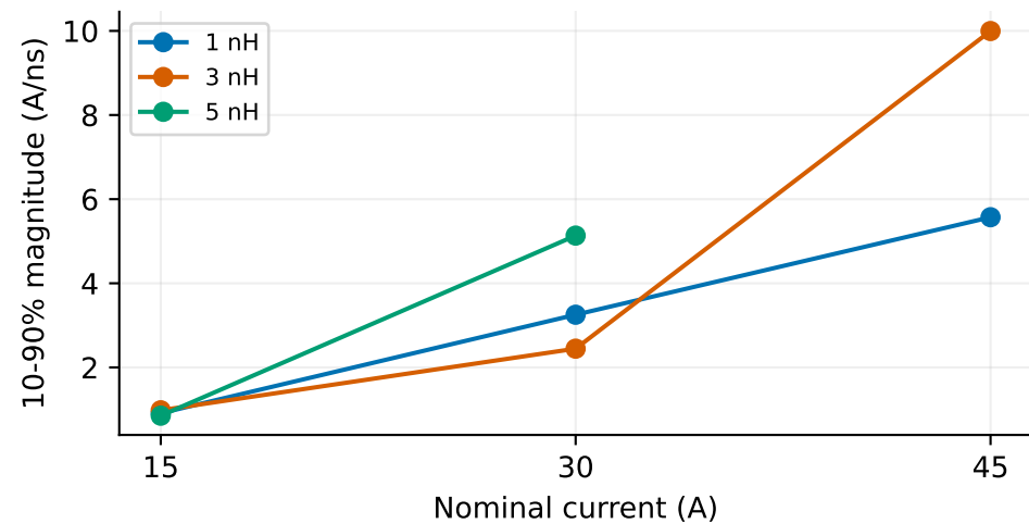
First turn-off terminal-current fall
