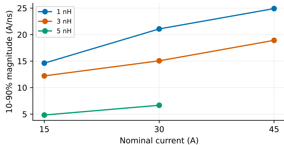
Turn-on terminal-current rise
