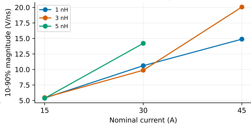
First turn-off terminal-current fall
