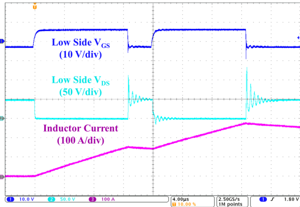
Fig. 7. Hardware DPT waveforms of the GaN module at 277 A
