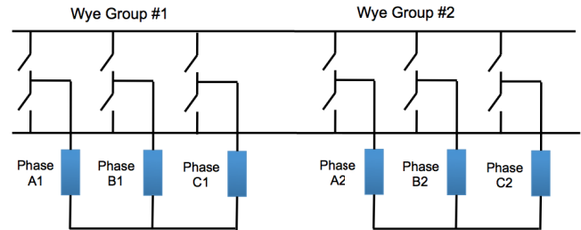
Figure 3: Basic 6-phase IMMD demonstrator drive configuration with two three-phase floating wye subcircuits and shared dc bus
