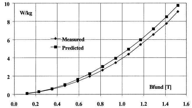
Fig. 7. Comparison between the measured and the predicted losses on the 8065 material with PWM supply versus fundamental flux density (switching frequency = 1 kHz; modulation index = 0.45; fundamental frequency 50 Hz).
