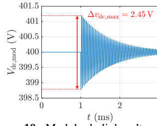
Figure 10: Module dc link voltage V_{dc,mod} for a load step from 0 A to 2 A, L_c = 7.5 \mu\text{H} , C_{dc,mod} = 10 \mu\text{F} , ESR = 10 \text{ m}\Omega .
