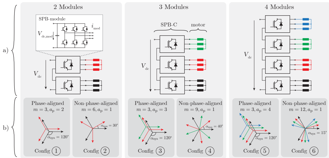
Figure 2: a) SPB-C with 2, 3, and 4 SPB-modules connected to motor windings [2]. b) For each SPB-C, two configurations of the magnetic winding axes are shown with m phases and a_p phase-aligned winding systems.
