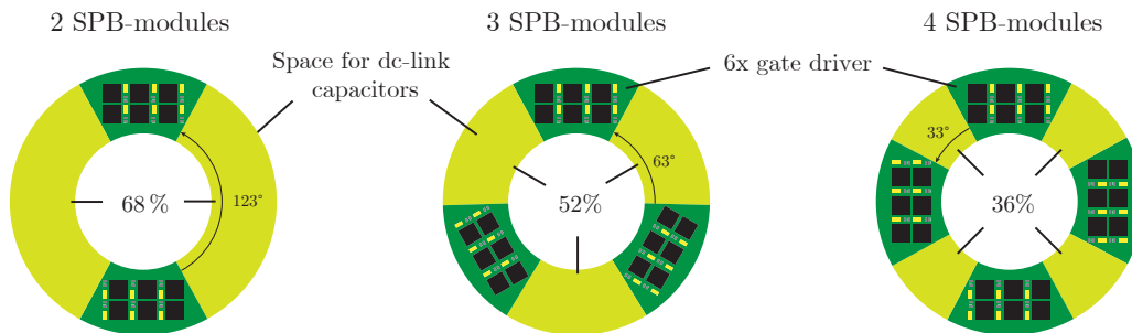
Figure 11: PCB-topside of a SPB-C with 2, 3, and 4 SPB-modules for estimating the PCB area available for dc-link capacitors. Transistors are mounted on the bottom-side. The used gate-driver dimensions result from gate-driver IEDS5663H (Infineon).
