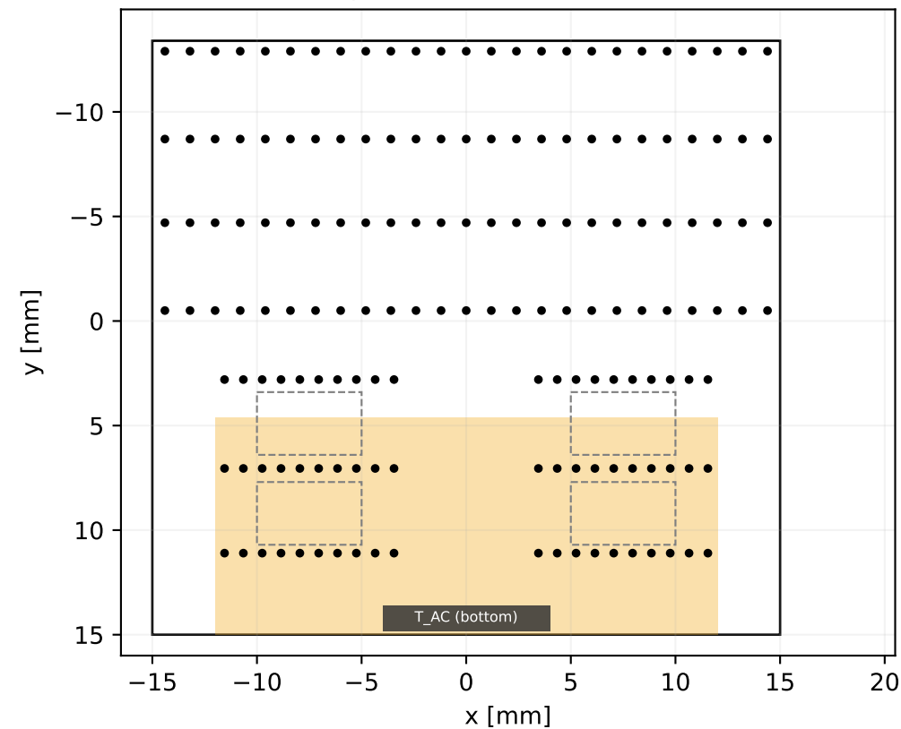
L4: AC plane, AC terminal bottom centre
