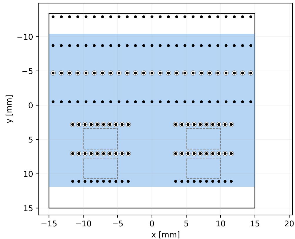
L2: DC- plane (anti-pads for DC+ / AC vias)
