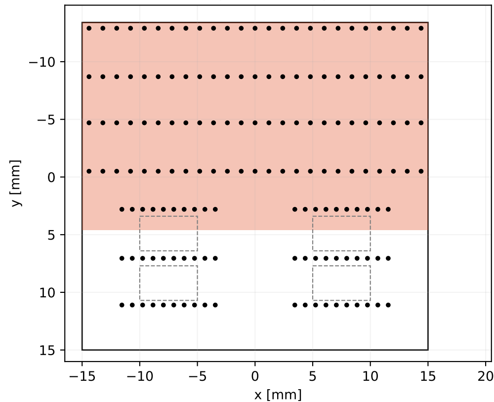
L3: DC+ plane (bank strips -&gt; cells)
