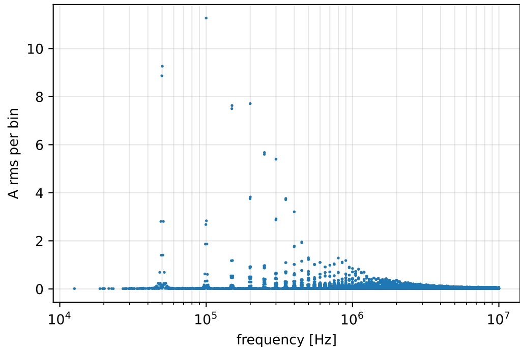
Leg ripple current spectrum, M = 1 , \cos \phi = 1 , 50 kHz
