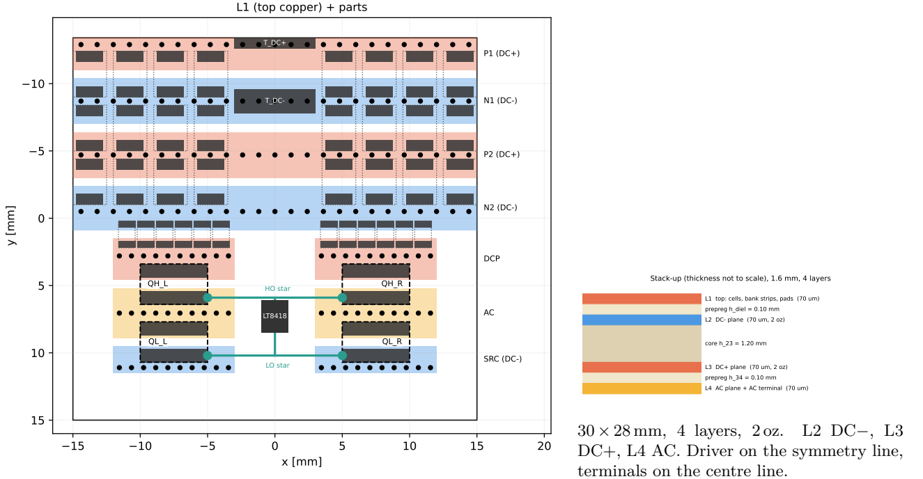
Figure 3: Building-block layout (generated from the same geometry as the Q3D model).
