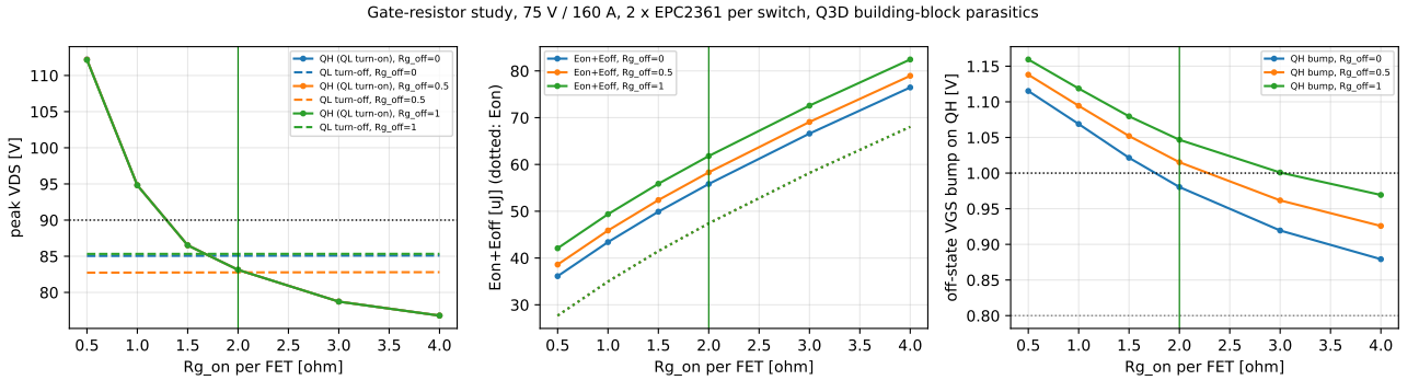
Figure 4: Gate-resistor study (LTspice with Q3D parasitics). Selected R_{g,\text{on}} = 2 \Omega , R_{g,\text{off}} = 0 \Omega : QH 83.1 V, QL 85.1 V, bump 0.98 V. EPC’s four-parallel motor-drive board uses much larger values (10 \Omega on / 2 \Omega off) because it deliberately limits dv/dt for the motor; a DPT-oriented power stage can switch faster.
