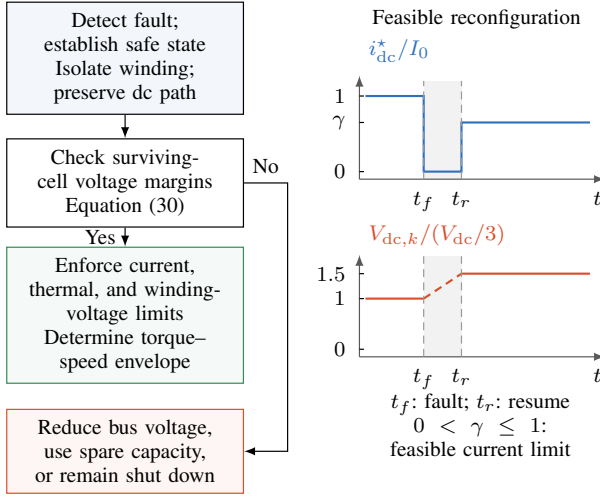
Fig. 15. Post-fault feasibility assessment with illustrative waveforms for the feasible branch. The dc-current command is temporarily set to zero and restored to \gamma I_0 , subject to operating limits. For a fixed bus, changing from three to two active cells raises the balanced surviving-cell voltage from 1 to 1.5 p.u. (400 to 600 V for a 1200-V bus). Shading marks the protection/reconfiguration interval; the dashed voltage connection indicates a change of steady-state level, not a predicted capacitor-voltage trajectory. Current derating does not remove the increased blocking-voltage requirement.
