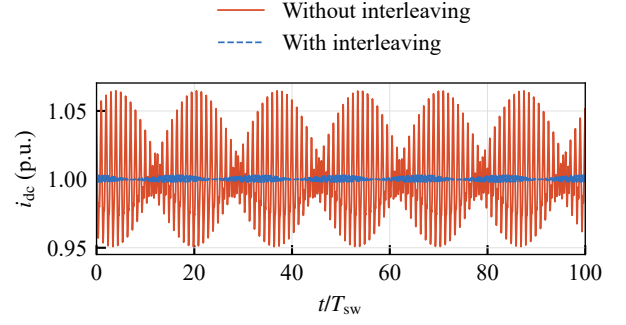
Fig. 9. Analytical steady-state shared dc-link current for three identical SPB cells with ideal natural SPWM over one fundamental period. Parameters are M = 0.85 , power-factor angle 20^\circ , f_{sw}/f_1 = 100 , L_b C/T_{sw}^2 = 0.85 , and R_b C/T_{sw} = 2.5 . Exact switching-interval Fourier integrals are propagated through (12), retaining 8000 fundamental harmonics. Both averages are 1 p.u.; ripple RMS is 0.0281 p.u. without interleaving and 0.00126 p.u. with uniform interleaving. These are ideal-model predictions, not measurements.
