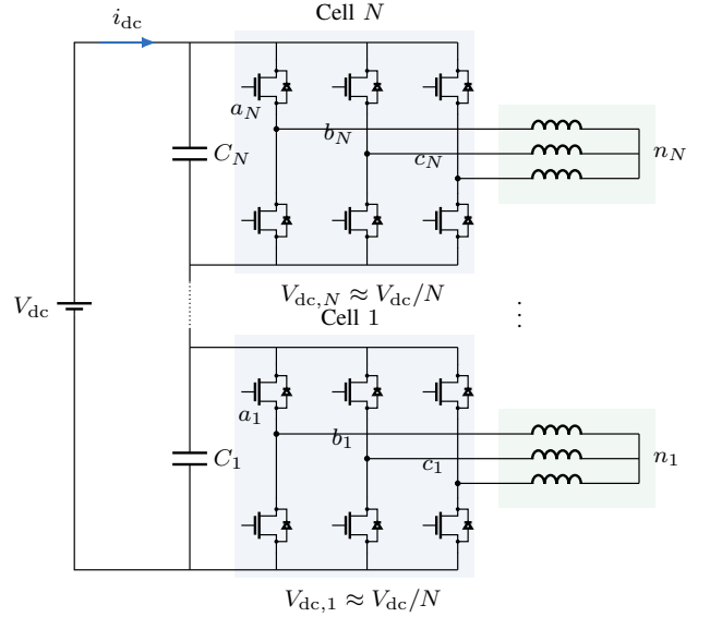
Fig. 5. Switch-level realization of the SPB dc-ac stage for two representative cells (Cell 1 and Cell N ; cells 2, \dots, N-1 elided). The common series current i_{dc} (2) flows through every cell, giving each cell the dc-side power p_{dc,k} = V_{dc,k} i_{dc} (3).
