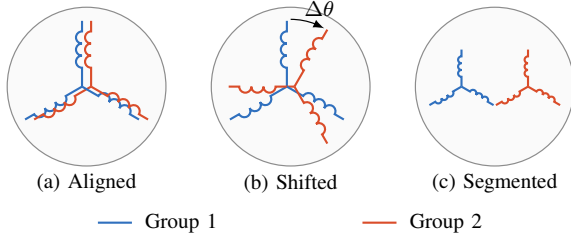
Fig. 6. Schematic comparison of winding-group spatial arrangements, each coil marking one phase axis of winding group 1 (blue) or group 2 (red): (a) aligned groups (parallel phase axes), (b) spatially shifted groups (offset by \Delta\theta ), and (c) physically segmented stator modules.
