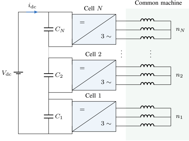
Fig. 3. Conceptual architecture of an N -cell SPB traction drive: series-connected local dc-link capacitors, series-connected three-phase two-level bridge cells, and their electrically separated machine winding groups.
