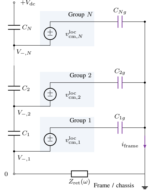
Fig. 10. Lumped common-mode equivalent of the SPB stack. Series dc-link capacitors C_k establish the rail offsets V_{-,k} ; each voltage source represents v_{cm,k}^{loc} = (v_{aN_k} + v_{bN_k} + v_{cN_k})/3 . The group-to-frame capacitance C_{kg} couples this local source and its rail offset to the chassis. Z_{ret}(\omega) represents the installation-dependent return path to the dc reference, not an assumed galvanic bond. Differential-mode winding circuits and the rotor/bearing network are omitted.
