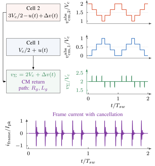
Fig. 11. Nonideal two-cell common-mode cancellation over two switching periods. Small transition misalignment produces narrow residuals in v_{\Sigma} ( t_d/T_{sw} = 0.003 , t_r/T_{sw} = 0.004 ). Their polarities follow the three rising and three falling cell-voltage transitions; unequal dv/dt can also produce residuals. The lower plot shows damped frame current with cancellation, normalized to its own peak I_{pk} . For equal winding-to-frame capacitances C_g and a shared frame-to-ground return impedance R_g + sL_g , I_{\text{frame}}(s)/V_{\Sigma}(s) = sC_g/(1 + 2R_gC_g s + 2L_gC_g s^2) . The illustrative resonance has f_0/f_{sw} = 65 and damping ratio \zeta = 0.22 . Each residual excites alternating-polarity current ringing. This lumped-model illustration excludes shaft charging and bearing-film breakdown; it is not a bearing-discharge prediction.
