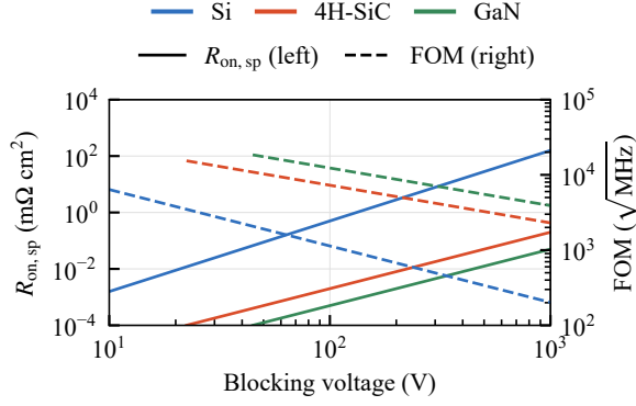
Fig. 2. Ideal one-dimensional unipolar specific on-state resistance R_{on,sp} (solid, left axis) and the resulting high-frequency figure of merit FOM = 1/\sqrt{R_{on,sp}C_{oss,sp}} (dashed, right axis), in \sqrt{\text{MHz}} – the product R_{on,sp}C_{oss,sp} is an area-independent RC time constant, versus blocking voltage for Si, 4H-SiC, and GaN.
