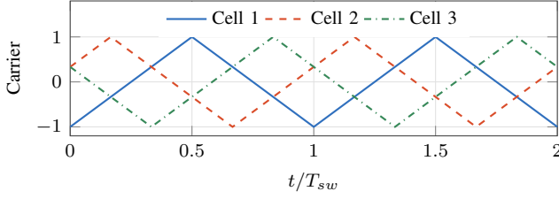
Fig. 8. Uniform carrier interleaving for N = 3 , with phase offsets 0, 2\pi/3 , and 4\pi/3 . Analytically generated triangular carriers.
