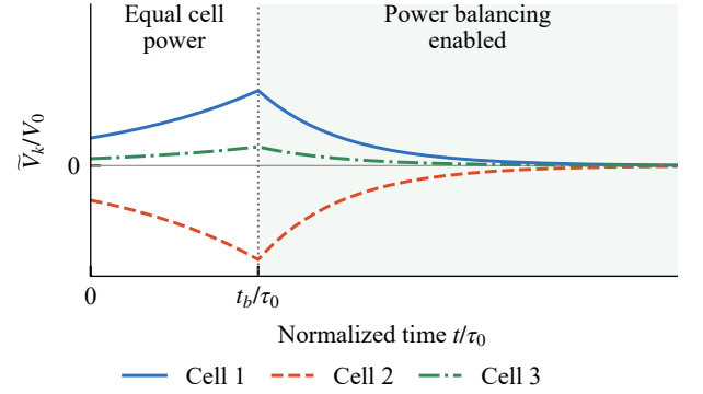
Fig. 12. Conceptual analytical illustration of voltage balancing for three cells during motoring, based on (20) and [45]. Small deviations from the mean grow under equal constant cell powers. Enabling differential power balancing at t_b makes them decay toward zero while \sum_k \Delta P_k = 0 . Time is normalized by \tau_0 = CV_0/I_{dc,0} ; amplitudes and gain are illustrative, not a hardware transient or a prediction of settling time.
