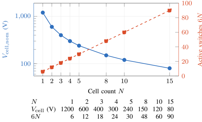
Fig. 13. Cell-count scaling for a 1200-V dc link: nominal cell voltage V_{\text{cell,nom}} = V_{\text{dc}}/N (blue circles, left logarithmic axis) and active switch positions 6N (red squares, right linear axis). The table gives the values at each design point. Illustrative device classes include 1700–2000-V SiC for N = 1 , 650-V GaN/SiC for N = 3 , and 100-V GaN or silicon MOSFETs for N = 15 , subject to the required blocking-voltage margin. Device parallelization is excluded.
