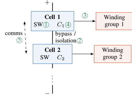
Fig. 14. Simplified SPB converter-machine structure with fault locations ①–⑤ annotated, corresponding in order to the rows of Table V.
