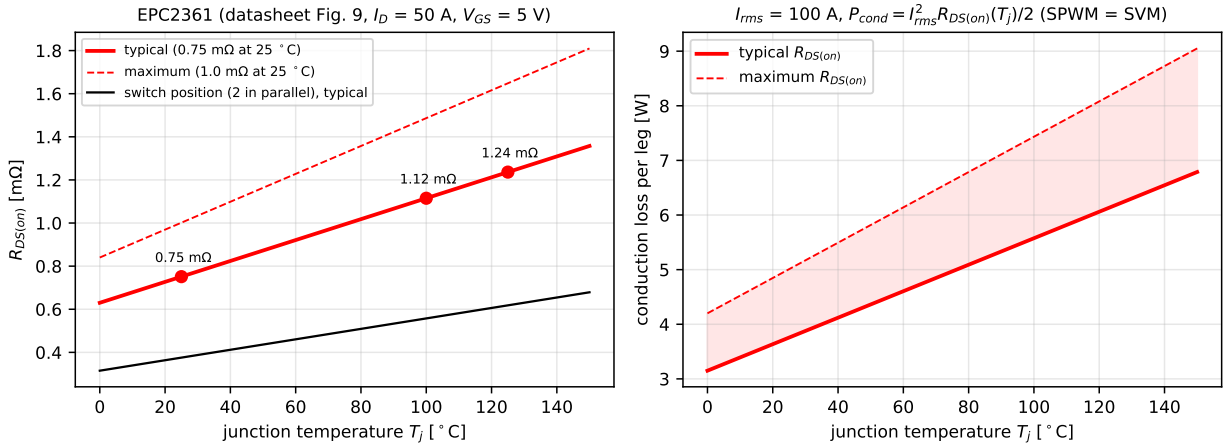
Figure 11: Left: R_{DS(on)} of EPC2361 versus junction temperature (datasheet Fig. 9, linear from 0.84 to 1.81\times the 25 ^\circ\text{C} value between 0 and 150 ^\circ\text{C} ). Right: conduction loss per leg at 100 A rms ; identical for SPWM and SVM.
