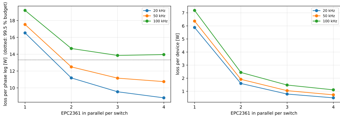
Figure 6: Loss per leg (left) and per device (right) versus devices per switch. The switching energy is scaled from the n = 2 LTspice E(i) fit.
