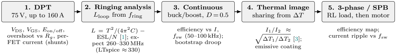
Figure 29: Validation sequence and what each step verifies.
