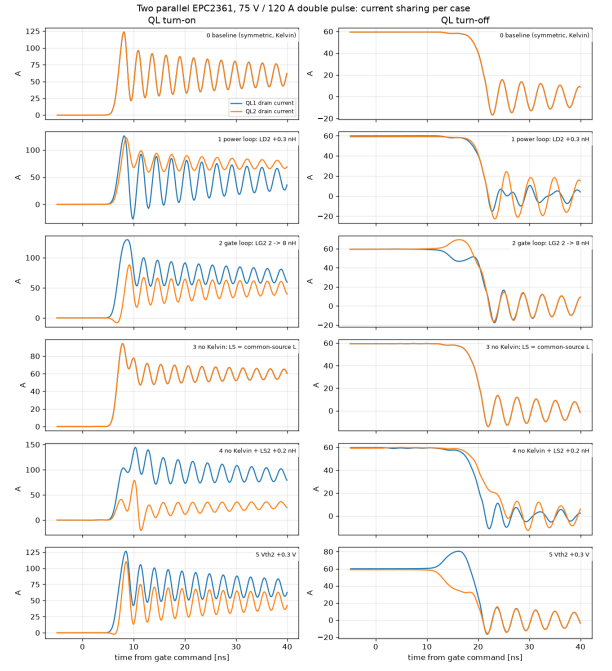
Figure 22: Waveforms of the six cases.
