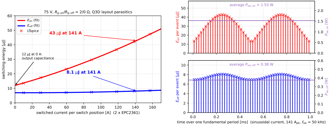
Figure 9: Left: switching energies of one switch position ( 2 \times \text{EPC2361} ) versus current: 43 \mu\text{J} ( E_{on} ) and 8.1 \mu\text{J} ( E_{off} ) at the rated peak of 141 A. Right: energy of each switching event over one fundamental period for a sinusoidal 100 \text{ A}_{rms} current at 50 kHz (fundamental 1 kHz for display); the averages give P_{sw,on} = 1.53 \text{ W} and P_{sw,off} = 0.38 \text{ W} . The same result holds for SPWM and SVM, since every leg switches once per period at the instantaneous current.
