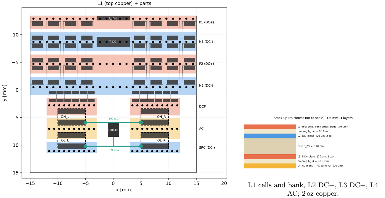
Figure 16: Layout generated from the same geometry as the Q3D model.
