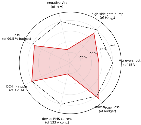
Figure 28: Utilisation of each constraint (1 = limit).
