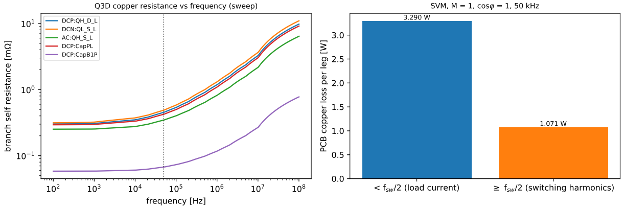
Figure 7: Left: Q3D copper resistance of the main branches versus frequency. Right: copper loss per leg split into the load-current part and the switching-harmonic part (SVM, M = 1 , \cos \varphi = 1 , 50 kHz).
