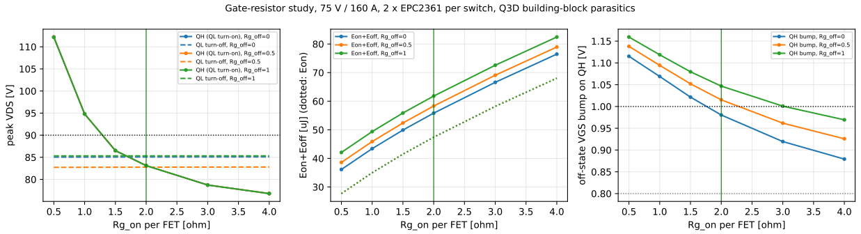
Figure 20: LTspice R_g study at 160\text{ A} with the Q3D parasitics. Selected: 2/0\Omega , giving QH 83.1\text{ V} , QL 85.1\text{ V} and a gate bump of 0.98\text{ V} .
