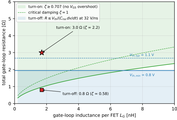
Figure 19: Gate-resistor design window for EPC2361 ( C_{iss} = 3.6\text{ nF} , C_{rss} = 13\text{ pF} ).
