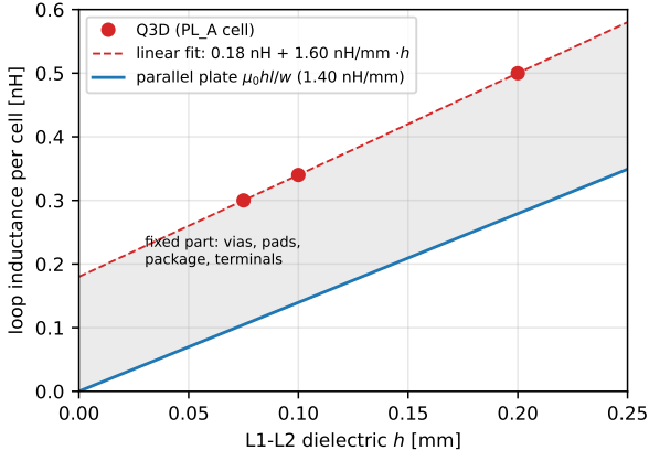
Figure 15: Loop inductance per cell versus the L1–L2 dielectric: analytical slope versus Q3D.
