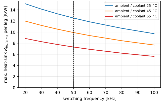
Figure 26: Maximum heat-sink resistance per leg for T_j \leq 125^\circ\text{C} .
