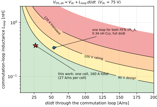
Figure 17: First-order overshoot map V_{DS,pk} = V_{dc} + L_{loop} di/dt . The operating point uses the effective di/dt through one cell (27 A/ns) that reproduces the LTspice peak at 160 A. At this di/dt the 90 V design limit allows L_{loop} \leq 0.56 nH per cell, which leaves room for the package and routing additions. A single loop carrying both FETs (PL_A) sees the full di/dt and would be at the 100 V rating.
