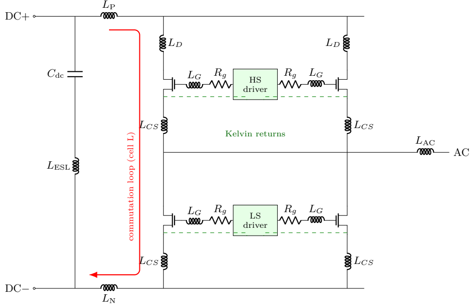
Figure 4: Equivalent circuit of the building block with the parasitic elements extracted by Q3D. The mirrored layout makes every left element equal to its right counterpart. L_{CS} is only the package and pad part because the gate loops return through Kelvin paths.
