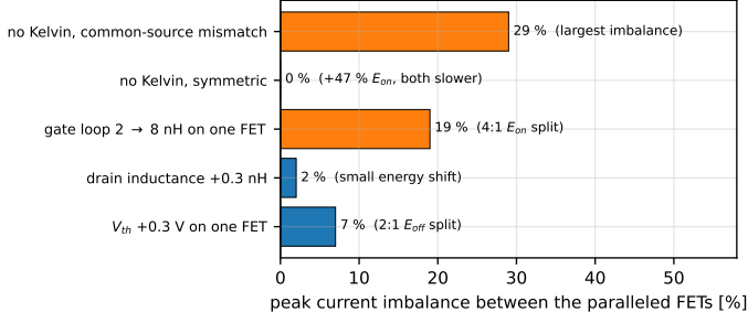
Figure 21: Sensitivity of the dynamic current imbalance (75 V, 120 A, 2 \times EPC2361).
