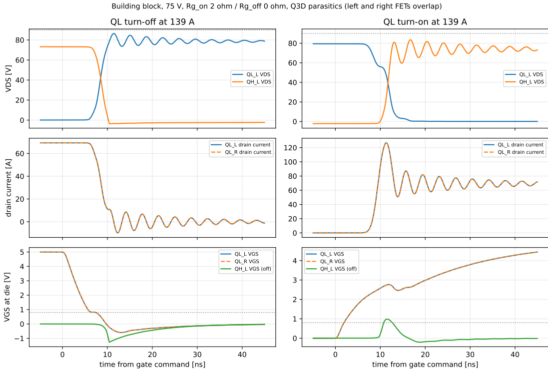
Figure 23: Building-block switching at the rated peak current. The left and right FET currents overlap.
