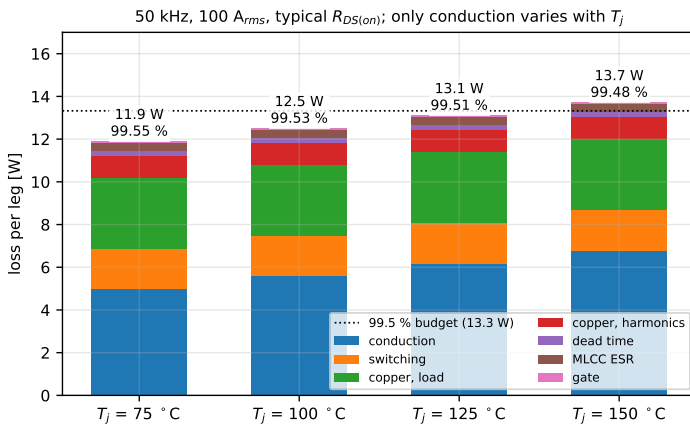
Figure 12: Loss and efficiency per leg versus junction temperature at 50 kHz. With typical devices the 99.5% target holds up to about 130 ^\circ\text{C} ; with maximum R_{DS(on)} it is missed above about 67 ^\circ\text{C} .
