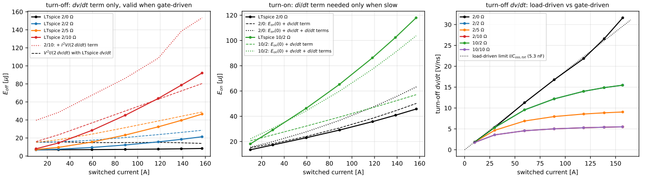
Figure 14: Left: E_{off} (solid) against V^2 I / (2 dv/dt) with the simulated dv/dt (dashed); the dotted curve adds the I^2 V / (2 di/dt) term for 2/10 \Omega . Centre: E_{on} against E_{on}(0) plus the overlap terms. Right: turn-off dv/dt ; the dotted line is the load-driven limit I/C_{oss,tot} .
