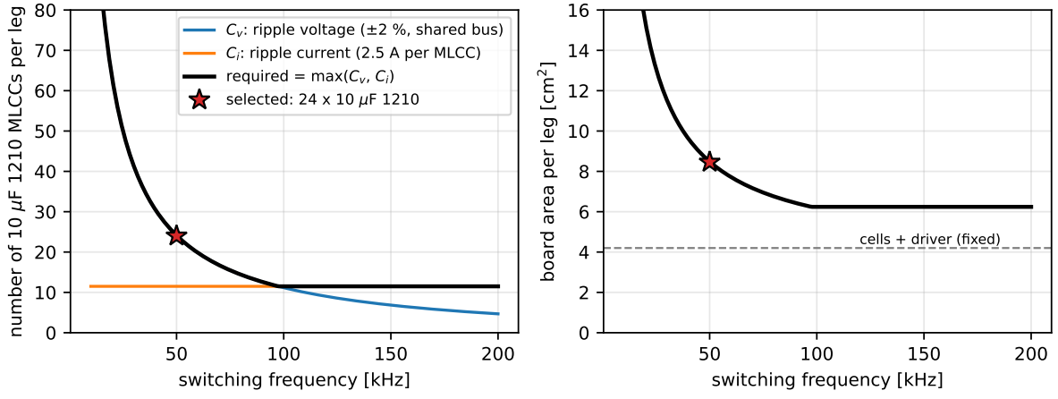
Figure 24: DC-link design space: MLCC count per leg (left) and resulting board area (right) versus f_{sw} .
