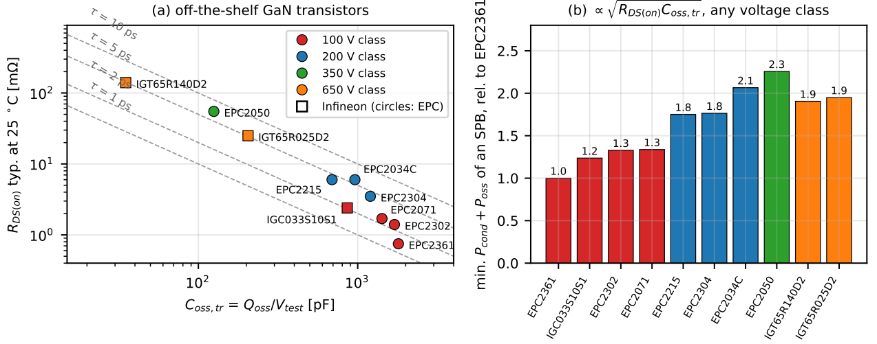
Figure 5: (a) Typical R_{DS(on)} against C_{oss,tr} = Q_{oss}/V_{test} of off-the-shelf GaN transistors (datasheets in Datasheet/ ), with lines of constant \tau . (b) Minimum conduction plus output-charge loss of an 800 V SPB at 100 A rms and 50 kHz relative to EPC2361.
