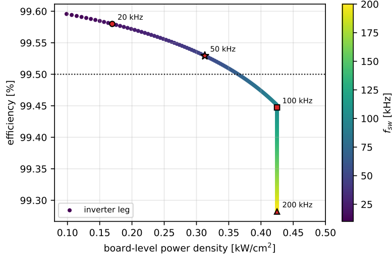
Figure 27: Efficiency versus board-level power density with f_{sw} as the parameter (10–200 kHz), inverter leg only.
