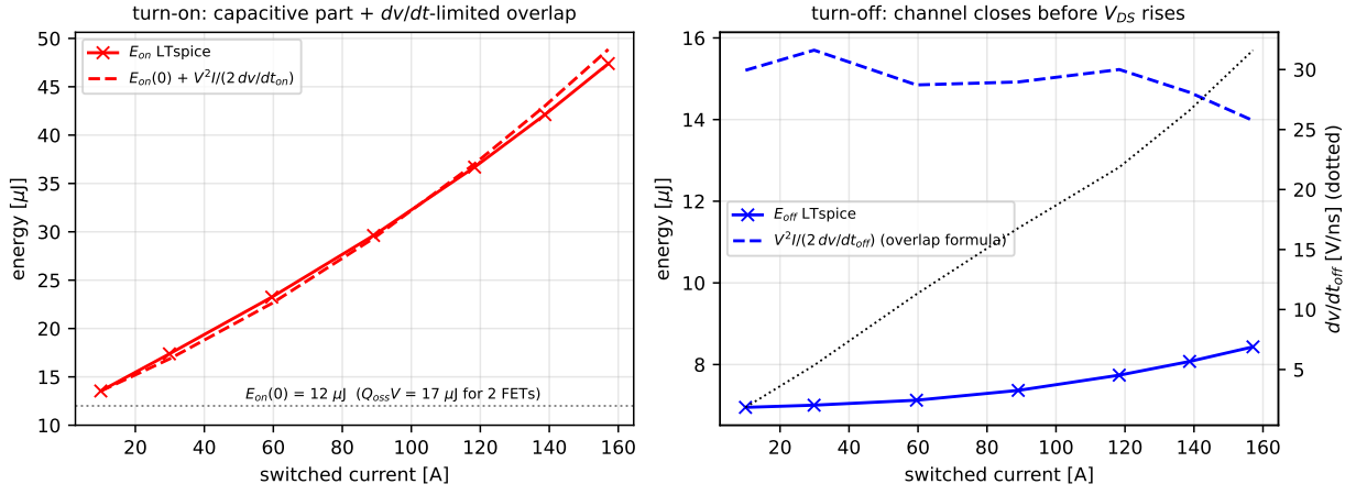
Figure 10: Decomposition of the switching energy. Turn-on: a current-independent output-capacitance part ( E_{on}(0) = 12 \mu\text{J} , of the order of Q_{oss} V = 17 \mu\text{J} for two FETs) plus an overlap part that follows V^2 I / (2 dv/dt) closely (37 vs. 35 \mu\text{J} at 157 A, dv/dt_{on} = 12 \text{ V/ns} ). Turn-off: the classical overlap formula overestimates by about 2\times (14 vs. 8.4 \mu\text{J} ) because the GaN channel closes before V_{DS} rises and the load current charges C_{oss} ; dv/dt_{off} (dotted) rises with current up to 32 V/ns.
