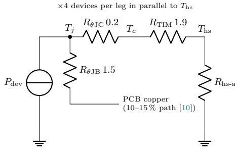
Figure 25: Thermal network per device.
