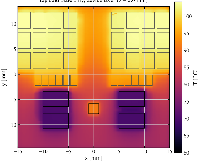
top cold plate only, device layer ( z = 2.0 mm)
