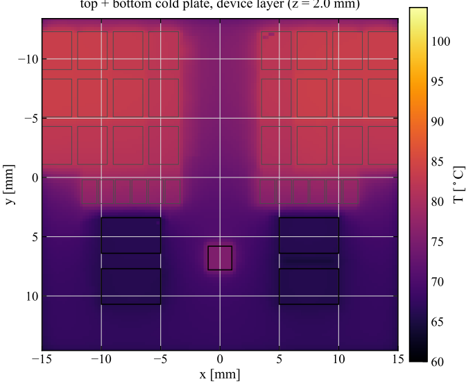
top + bottom cold plate, device layer ( z = 2.0 mm)
