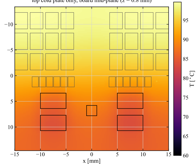
top cold plate only, board mid-plane ( z = 0.8 mm)
