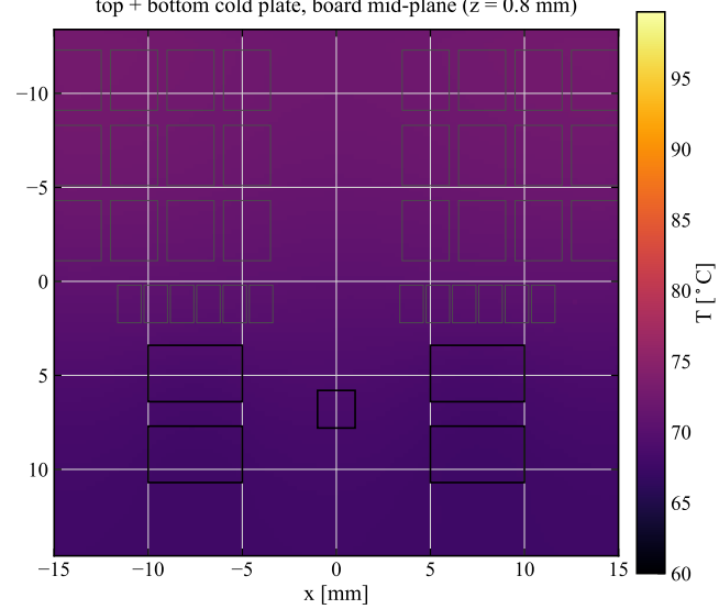
top + bottom cold plate, board mid-plane ( z = 0.8 mm)
