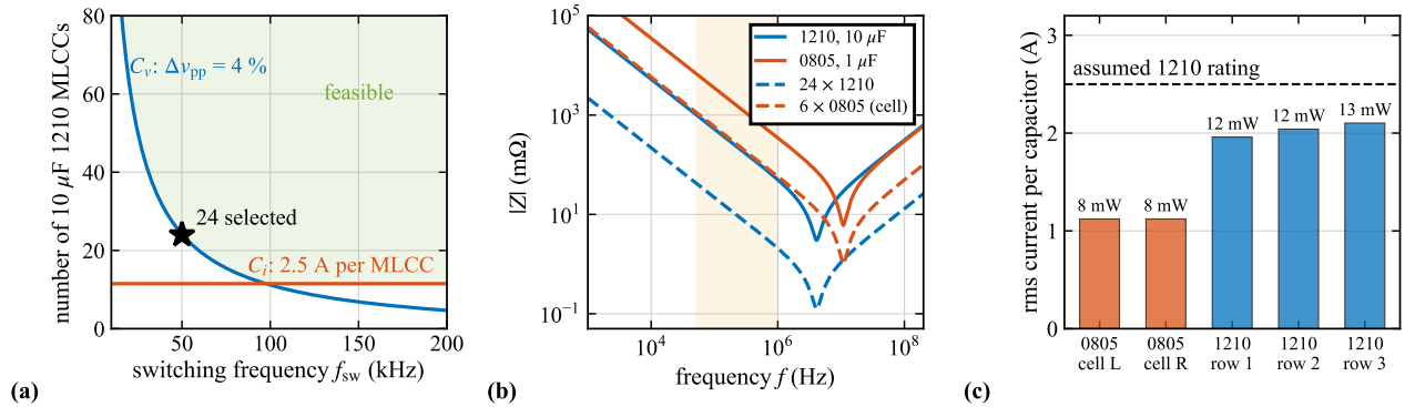
Fig. 6. DC-link design of the building block. (a) Number of 10 \mu F 1210 MLCCs per leg against switching frequency, required for a 4 % peak-to-peak voltage ripple on a three-leg submodule bus ( C_v , blue) and for an rms current of 2.5 A per capacitor ( C_i , red); the shaded area is feasible, the star marks the selected bank. (b) Impedance magnitude of single capacitors (solid) and of the bank and the local group of one cell (dashed) from the C_{eff} -ESR-ESL model; the shaded band covers the switching frequency and its first harmonics. (c) RMS ripple current and loss per capacitor at the rated point, from the frequency-domain network of the Q3D board impedances and the capacitor models.
