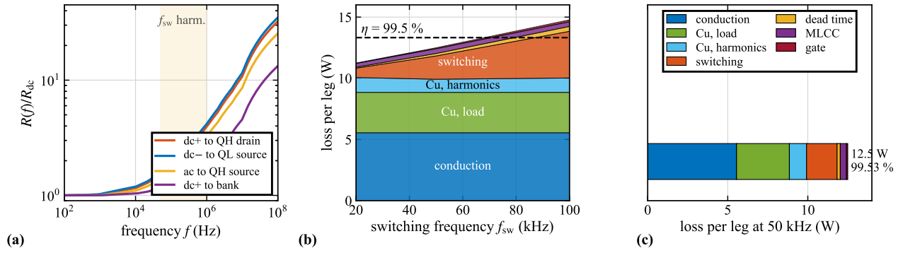
Fig. 9. Losses of the building block at the rated point (75 V, 100 A rms , M = 1 , typical R_{DS(on)} at 100 °C). (a) Q3D resistance of the main board branches against frequency, normalized to the dc value; the shaded band covers the switching frequency and its first harmonics. (b) Loss per leg against switching frequency with the efficiency target. (c) Loss breakdown at 50 kHz; conduction and copper loss together account for about 80 %.
