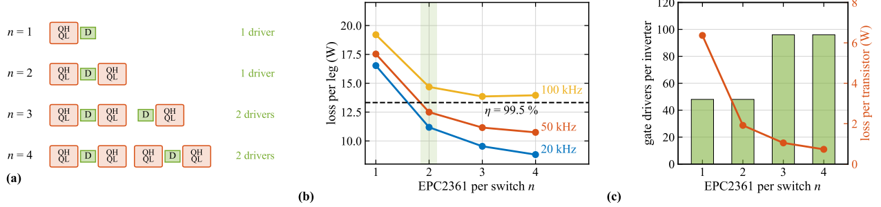
Fig. 5. Number of EPC2361 per switch. (a) Scaling of the layout concept: two-device cells (red) with one star-connected half-bridge driver (D, green) per pair; three devices per switch need a second driver, four are built from two two-device structures. (b) Loss per leg at the rated point (75 V, 100 A_{rms} , M = 1 , typical R_{DS(on)} at 100^\circ C , including copper and capacitor losses) for 20, 50 and 100 kHz; the dashed line is the 99.5 % target. (c) Gate drivers of the complete 1200 V inverter (16 submodules, 48 legs) and loss per transistor at 50 kHz.
