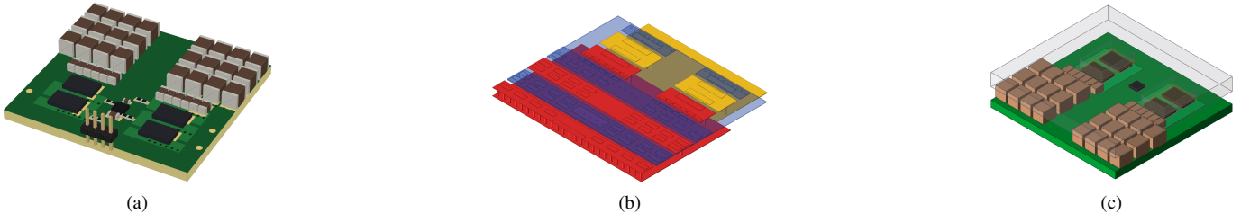
Fig. 4. One parametric geometry, three models. (a) KiCad placement with the component 3D models ( 30 \times 28.2 mm, four layers, 2 oz copper): MLCC bank (top), local MLCCs, the two mirrored cells with QH and QL, and the centre driver. (b) Ansys Q3D copper model with the dc+ (red), dc- (blue, transparent) and ac (yellow) nets and the via rows of the vertical loops. (c) Ansys Icepak model with gap pads, pedestals and the aluminium cold plate (shown above the board).
