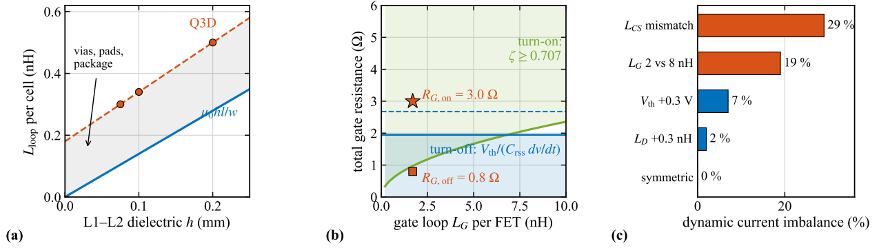
Fig. 7. Parasitic design of the building block. (a) Commutation-loop inductance per cell against the L1-L2 dielectric thickness h : Q3D extraction (circles, linear fit dashed) and parallel-plate estimate \mu_0 h l / w ; the shaded difference is the fixed contribution of vias, pads and package. (b) Gate-resistor design window per transistor: lower bound for critical damping of the gate loop at turn-on (green, \zeta \geq 0.707 ) and upper bound against Miller turn-on at turn-off (blue, solid for V_{th,min} = 0.8 V, dashed for 1.1 V), with the selected resistances at L_G = 1.7 nH. (c) Dynamic current imbalance of two paralleled EPC2361 (75 V, 120 A, LTspice) for one asymmetry at a time: common-source inductance mismatch without Kelvin connection, unequal gate loops, threshold-voltage spread and drain-path mismatch.
