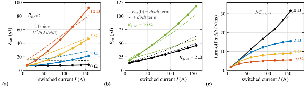
Fig. 8. Switching energies per switch position of the building block with slow switching (LTspice with the Q3D parasitics, 75 V, R_{g,\text{on}} and R_{g,\text{off}} external resistances). (a) Turn-off energy (solid) and voltage-overlap estimate V^2 I / (2 dv/dt) with the simulated dv/dt (dashed) for R_{g,\text{off}} = 0, 2, 5 and 10 \Omega ; the estimate fails below the critical resistance (3). (b) Turn-on energy for R_{g,\text{on}} = 2 and 10 \Omega against the current-independent part E_{\text{on}}(0) plus the voltage-overlap term (dashed) and plus the current-overlap term (dotted). (c) Turn-off dv/dt against the load-driven limit I/C_{\text{oss,tot}} (dotted): without external resistance the voltage rise is set by the load current, with 5–10 \Omega by the gate.
