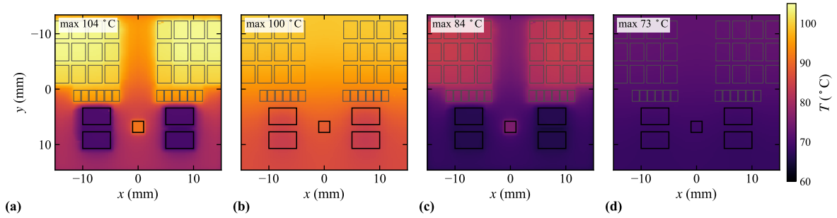
Fig. 10. Icepak temperature maps at the rated point (50 kHz) in the device layer ( z = 2.0 mm, including the air between components) and the board mid-plane. (a), (b) Cold plate on the transistors only. (c), (d) Additional bottom-side gap pad (3 W/mK) to a second plate at 60 °C. Outlines: transistors, MLCCs and driver.
