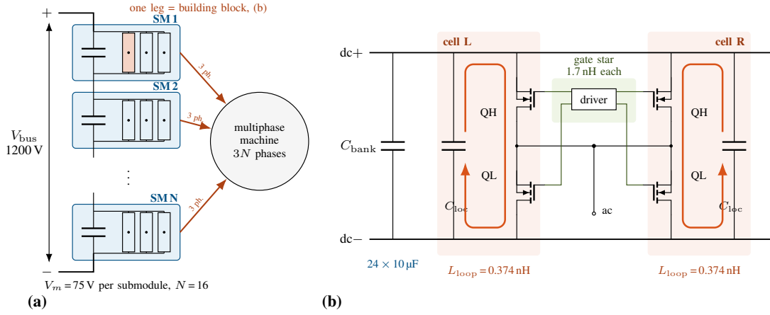
Fig. 1. (a) Stacked polyphase bridge (SPB) inverter: N three-phase submodules (SM) are connected in series on the dc side and feed the N three-phase winding sets of a multiphase machine; each submodule operates at V_m = V_{\text{bus}}/N . (b) Building block designed in this paper, i.e., one phase leg of a submodule: two mirror-symmetric commutation cells (red) with one high-side (QH) and one low-side (QL) EPC2361 each, so that two transistors are paralleled per switch, local MLCCs C_{\text{loc}} in every cell, a common MLCC bank C_{\text{bank}} and a centre gate driver (green) with equal, star-connected gate loops. The red arrows indicate the commutation loop of each cell (Q3D, including capacitor ESL).
