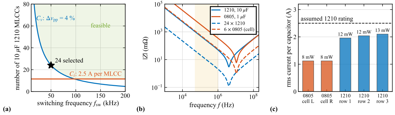
Fig. 7. DC-link design of the building block. (a) Number of 10 \mu\text{F} 1210 MLCCs per leg against switching frequency, required for a 4% peak-to-peak voltage ripple on a three-leg submodule bus ( C_v , blue) and for an rms current of 2.5 A per capacitor ( C_i , red); the shaded area is feasible, the star marks the selected bank. (b) Impedance magnitude of single capacitors (solid) and of the bank and the local group of one cell (dashed) from the C_{\text{eff}} –ESR–ESL model; the shaded band covers the switching frequency and its first harmonics. (c) RMS ripple current and loss per capacitor at the rated point, from the frequency-domain network of the Q3D board impedances and the capacitor models.
