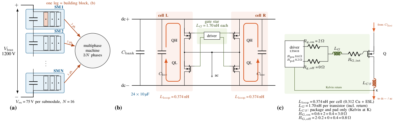
Fig. 1. (a) Stacked polyphase bridge (SPB) inverter: N three-phase submodules (SM) are connected in series on the dc side and feed the N three-phase winding sets of a multiphase machine; each submodule operates at V_m = V_{bus}/N . (b) Building block designed in this paper, i.e., one phase leg of a submodule: two mirror-symmetric commutation cells (red) with one high-side (QH) and one low-side (QL) EPC2361 each, so that two transistors are paralleled per switch, local MLCCs C_{loc} in every cell, a common MLCC bank C_{bank} and a centre gate driver (green) with equal, star-connected gate loops. The red arrows indicate the commutation loop of each cell. (c) Gate and power circuit of one transistor with the values used in this paper: external gate resistors R_{g,on} = 2\Omega and R_{g,off} = 0\Omega , driver pull-up and pull-down resistances, internal gate resistance R_{G,int} = 0.4\Omega , gate-loop inductance L_G (Q3D, gate path and Kelvin return), and the common-source inductance L_{CS} , which the Kelvin connection K at the source pad limits to the package and pad; the commutation loop L_{loop} is per cell (Q3D, copper plus capacitor ESL).
