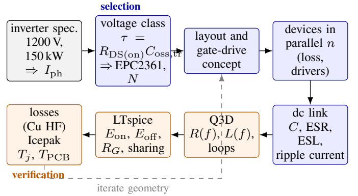
Fig. 2. Design procedure of the SPB building block: selection steps (blue) from the inverter specification to the dc link, followed by verification with one parametric geometry (orange), whose results feed back into the layout.
