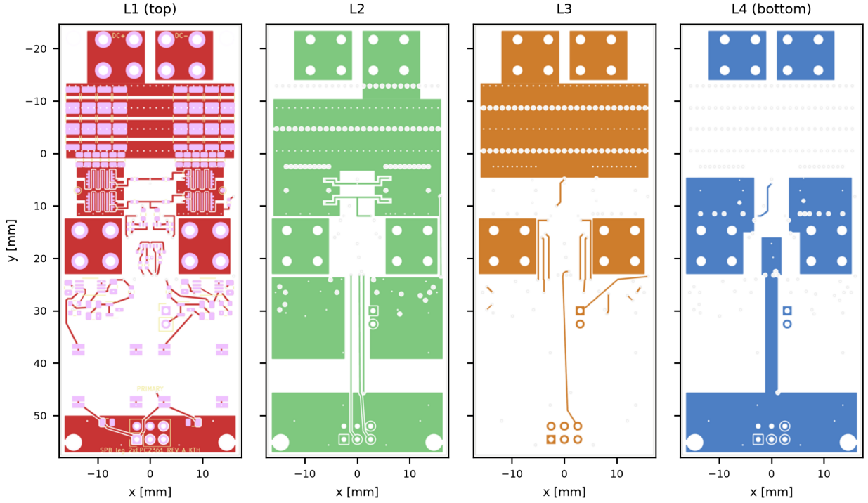
Figure 1: Copper layers of the Rev A board (top view on all layers). Red: L1, green: L2 (DC– return plane under the cells, VEE pours under the supply chains, GNDI at the bottom), orange: L3 (DC+ plane under the strips and the bank, supply columns), blue: L4 (switch-node plane, GNDI channel and bottom pour).
