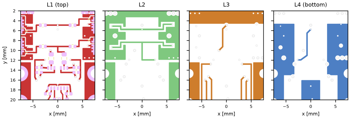
Figure 3: Driver corridor between the cells. L1: high-side star (upper row) and low-side star (lower row), each with two 0.5\text{ }\Omega ; the 0.75\text{ }\Omega common resistors above the 2EDF7275K; local decoupling to the left (A) and right (B) of the driver. L2: Kelvin collectors from the source-pad ends to the symmetry line in narrow keepouts of the DC- plane; the low-side collector continues to the B decoupling. L3: high-side trunk from the star via down the corridor; supply columns of both chains. L4: high-side Kelvin return directly under the L3 trunk inside the corridor keepout of the switch-node plane.
