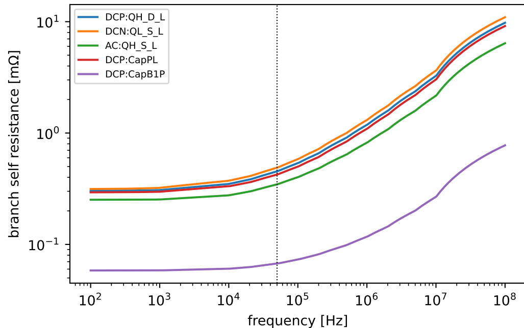
Q3D copper resistance vs frequency (sweep)
