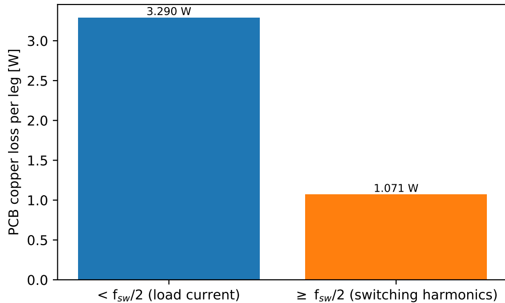
SVM, M = 1, cosφ = 1, 50 kHz
